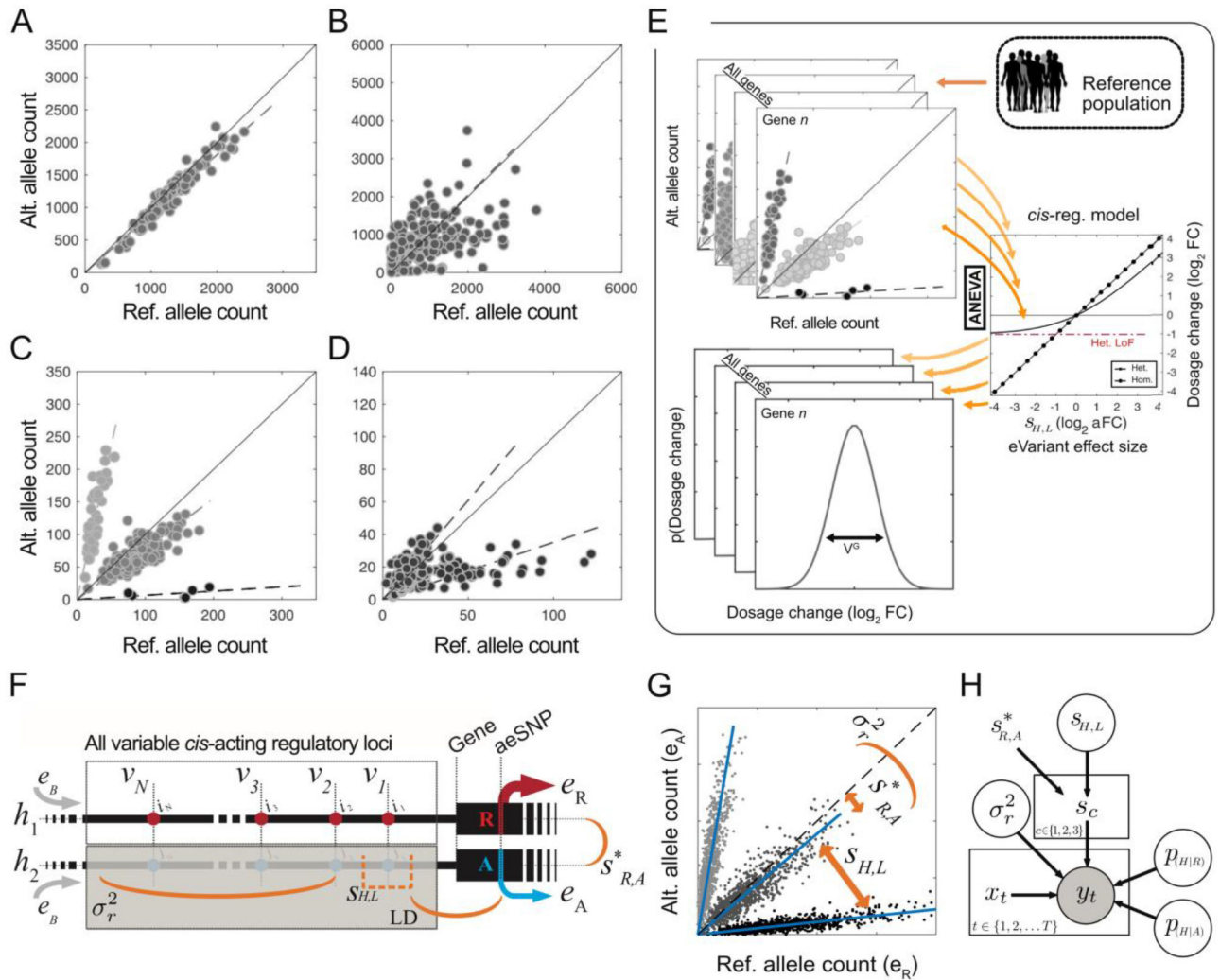
Figure 1: Cis-regulatory variation, allelic expression, and ANEVA.
