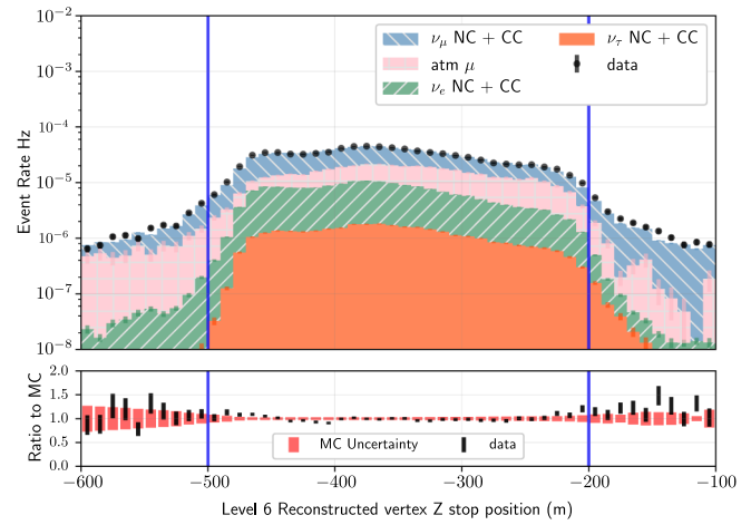
FIG. 30. (top) Distribution of stopping z_{\text{stop}} positions of the reconstructed track at level 6 (before cut applied). Each shaded color represents the stacked histogram from each event type. Black dots represents the data distribution. The vertical lines are the cut values; events between the two vertical lines are kept. MC events are weighted by world averaged best fit oscillation parameters. (bottom) Ratio of distribution from data to that from MC. Black error bars are the statistical fluctuation from data, whereas shaded red areas are the uncertainties from limited MC statistics.
