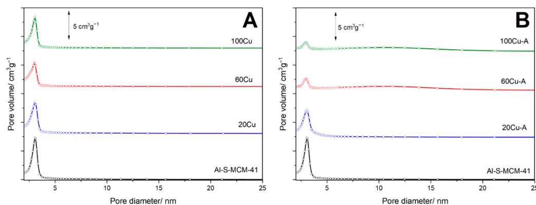
Figure 3. Pore size distributions of the of the Al-S-MCM-41 sample and its modifications with copper obtained by TIE (A) and TIE-NH 3 (B) methods.
