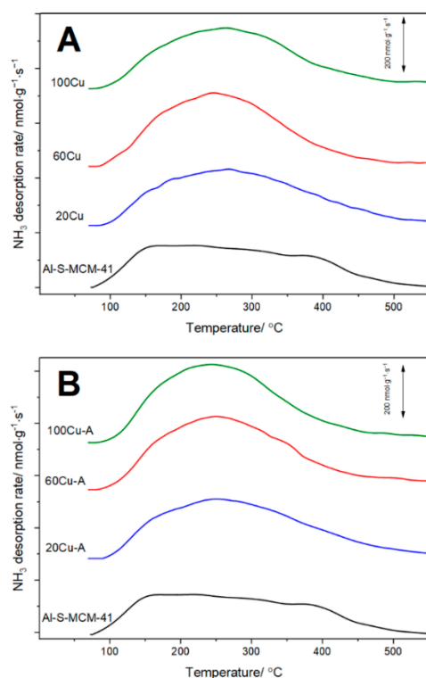
Figure 9. NH_3 -TPD profiles of the Al-S-MCM-41 sample modified with copper by TIE (A) and TIE- NH_3 (B) methods.
