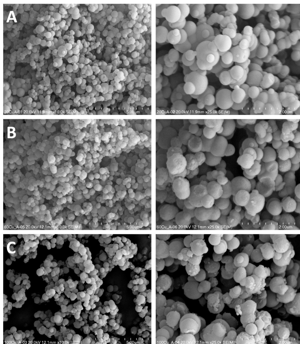
Figure 6. SEM images of the 20Cu-A (A), 60Cu-A (B) and 100Cu-A (C) samples at various magnifications.
