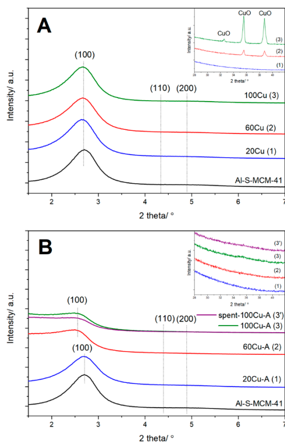
Figure 1. Powder X-ray diffractograms of the Al-S-MCM-41 sample and its modifications with copper obtained by TIE (A) and TIE-NH 3 (B) methods.
