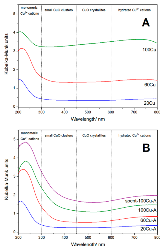
Figure 7. UV-vis-DR spectra of the Al-S-MCM-41 sample modified with copper by TIE (A) and TIE-NH 3 (B) methods.
