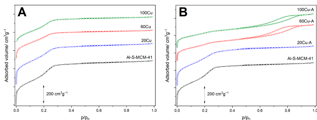
Figure 2. N 2 adsorption-desorption isotherms of the Al-S-MCM-41 sample and its modifications with copper obtained by TIE (A) and TIE-NH 3 (B) methods.
