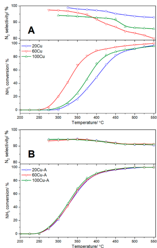
Figure 11. Temperature dependence of the ammonia conversion and N 2 selectivity in process of ammonia oxidation for the Al-S-MCM-41 sample modified with copper by TIE (A) and TIE-NH 3 (B) methods.
