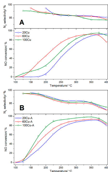
Figure 10. Temperature dependence of the NO conversion and N 2 selectivity in NH 3 -SCR for the Al-S-MCM-41 sample modified with copper by TIE (A) and TIE-NH 3 (B) methods.
