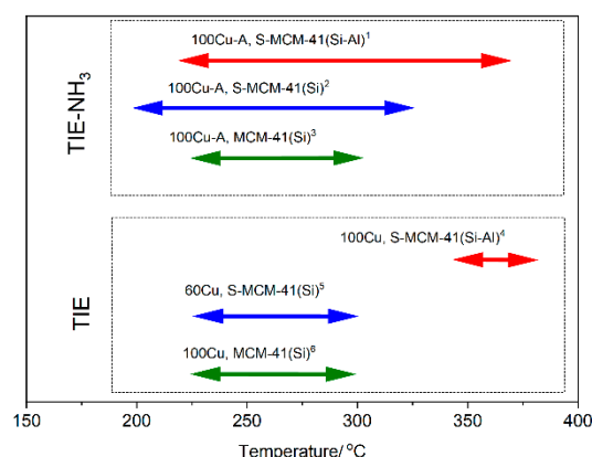
Figure 12. Comparison of the temperature ranges of the NO conversion over 90% for the most active catalysts obtained by TIE-NH 3 and TIE methods: 1 silica-alumina spherical MCM-41 modified with copper by TIE-NH 3 method, selectivity to N 2 (S N2 ) in this range above 95%, this studies; 2 pure silica spherical MCM-41 modified with copper by TIE-NH 3 method, S N2 > 98% [11]; 3 pure silica spherical MCM-41 modified with copper by TIE-NH 3 method, S N2 > 97% [12]; 4 silica-alumina spherical MCM-41 modified with copper by TIE method, S N2 > 95%, this work; 5 pure silica spherical MCM-41 modified with copper by TIE method, S N2 > 98% [11]; 6 pure silica spherical MCM-41 modified with copper by TIE method, S N2 > 97% [12].
