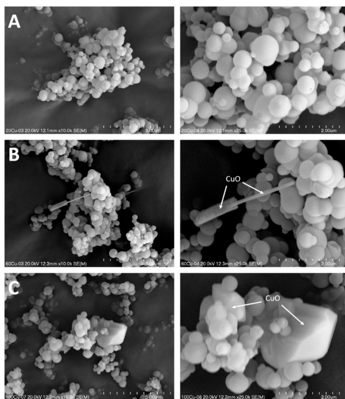
Figure 5. SEM images of the 20Cu (A), 60Cu (B) and 100Cu (C) samples at various magnifications.
