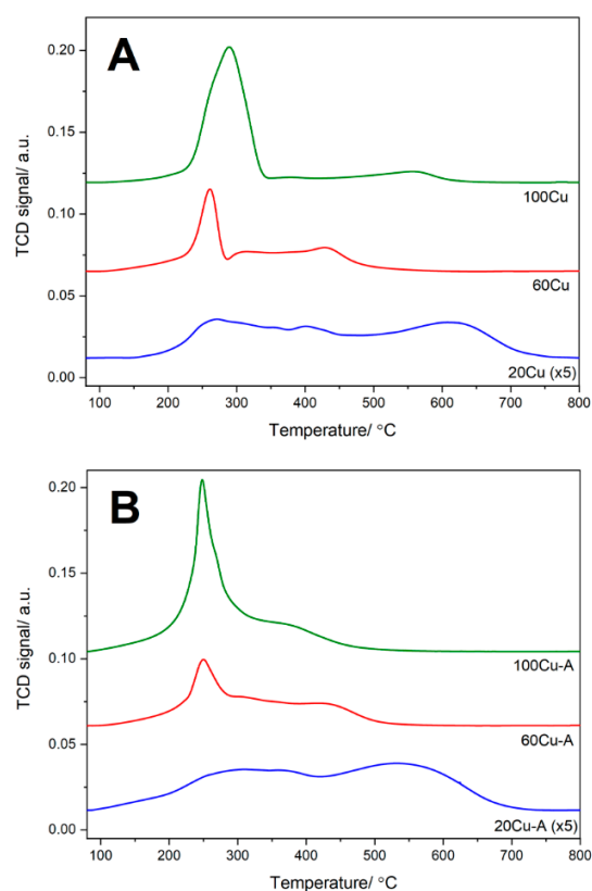
Figure 8. Results of H 2 -TPR studies of the Al-S-MCM-41 sample modified with copper by TIE (A) and TIE-NH 3 (B) methods.
