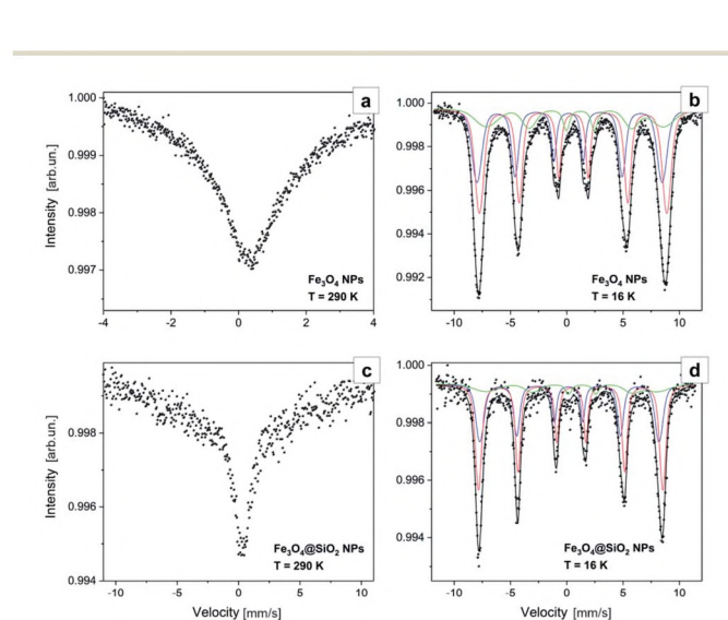
Fig. 7 Mössbauer spectra of the \text{Fe}_3\text{O}_4 NPs acquired at 290 K (a) and 16 K (b) and of the \text{Fe}_3\text{O}_4@\text{SiO}_2 NPs acquired at 290 K (c) and 16 K (d).
