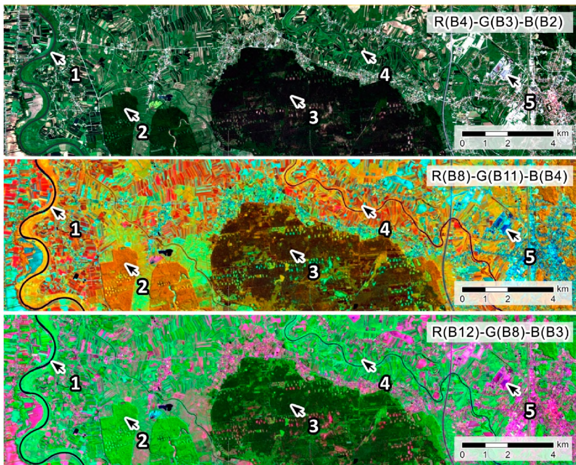
Figure 2. Five points that represent various land cover and land use classes on a satellite image of the same area, presented in three color band combinations. Satellite image acquired by Sentinel-2 at 6th June 2020.
