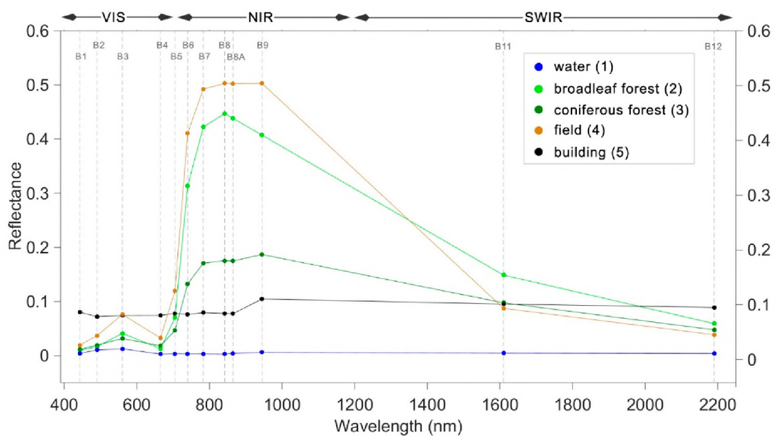
Figure 3. Spectral profiles of the points presented in Figure 2. In addition, the Sentinel-2 spectral bands are indicated (B1–B12) at the top of the plot.
