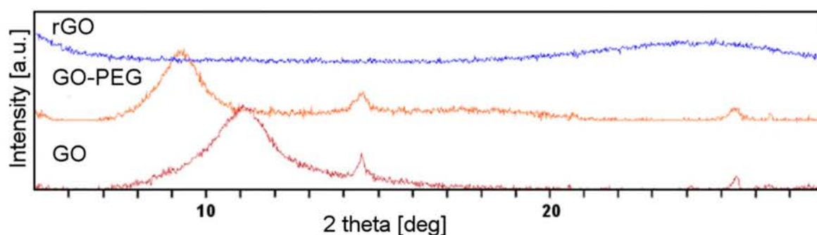
Figure 2. X-ray diffractometry (XRD) patterns of graphene oxide (GO), poly(ethylene glycol) grafted graphene oxide (GO-PEG) and reduced graphene oxide (rGO).
