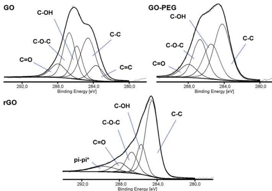
Figure 1. X-ray photoelectron spectroscopy (XPS) spectra (C1s) of graphene oxide (GO), poly(ethylene glycol) grafted graphene oxide (GO-PEG) and reduced graphene oxide (rGO).
