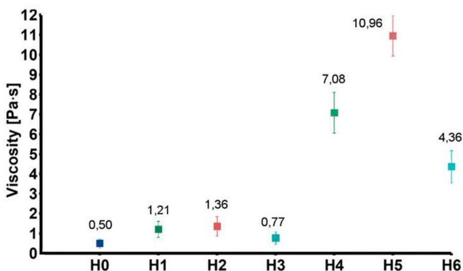
Figure 3. Viscosity of the tested solution (H0: chitosan (CS)) and dispersions (H1: CS/graphene oxide (GO); H2: CS/poly(ethylene glycol) grafted graphene oxide (GO-PEG); H3: CS/reduced graphene oxide (rGO); H4: CS/GO/hydroxyapatite (HAp); H5: CS/GO-PEG/HAp; H6: CS/rGO/HAp).
