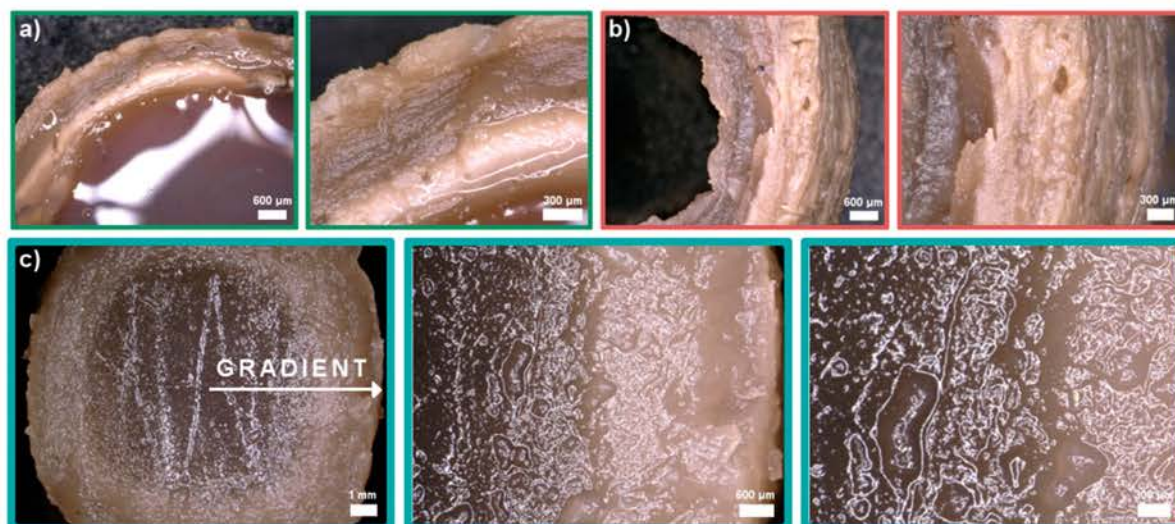
Figure 4. Digital microphotographs of chitosan/graphene oxide (H1) hydrogels obtained in three types of cross-linking solutions: (a) 5% TPP (sodium tripolyphosphate), 2 h + 10% NaOH, 10 min, (b) 5% TPP, 4 h + 10% NaOH, 10 min, (c) 0.5% TPP with 5% NaCl, 24h.
