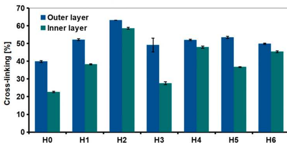
Figure 6. Degree of cross-linking in chitosan-based hydrogels (H0: chitosan (CS); H1: CS/graphene oxide (GO); H2: CS/poly(ethylene glycol) grafted graphene oxide (GO-PEG); H3: CS/reduced graphene oxide (rGO); H4: CS/GO/hydroxyapatite (HAp); H5: CS/GO-PEG/HAp; H6: CS/rGO/HAp) measured by ninhydrin assay.
