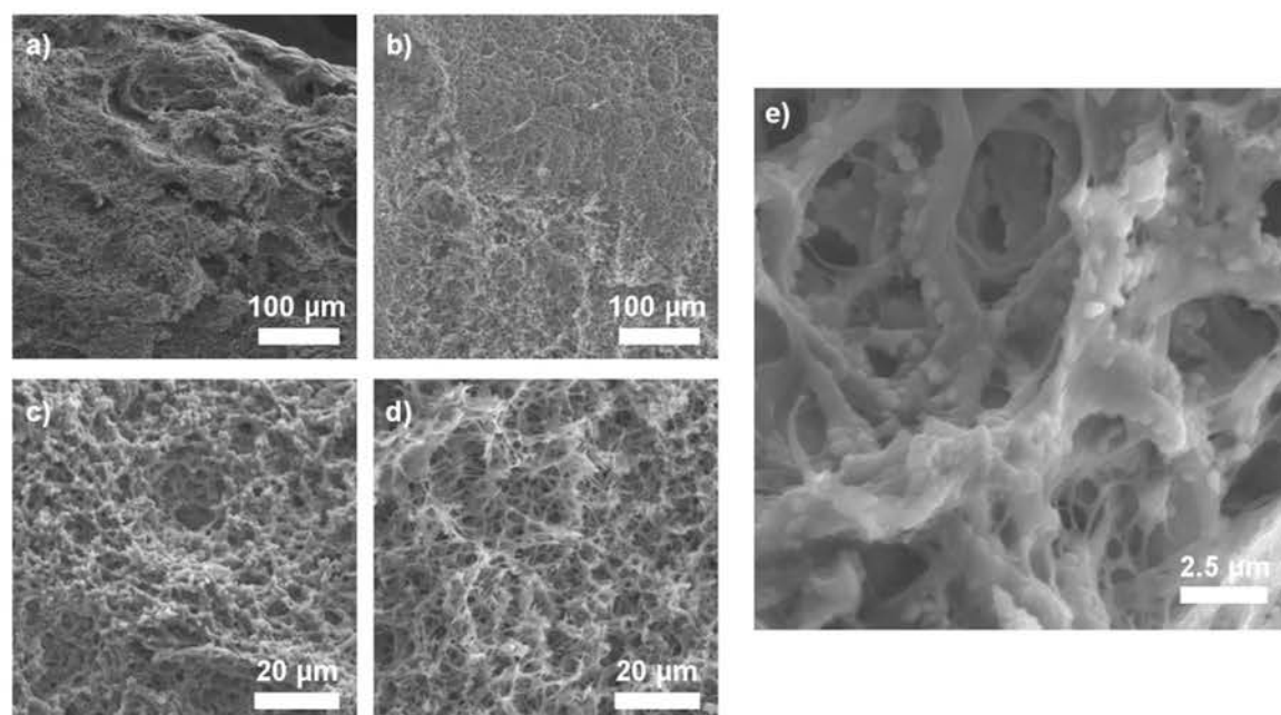
Figure 5. Representative SEM images of gradient hydrogels after freeze-drying (sample H5: chitosan/poly(ethylene glycol) grafted graphene oxide (GO-PEG)): (a) Edge of the sample, (b) Gradient inside, (c) Outer part, (d) Inner part, (e) Surface with visible hydroxyapatite (HAp) particles.
