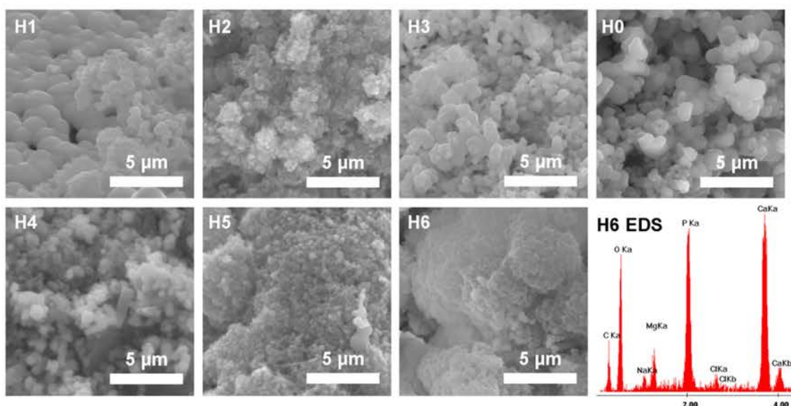
Figure 12. SEM (scanning electron microscopy) images of the hydrogels surface (H0: chitosan (CS); H1: CS/graphene oxide (GO); H2: CS/poly(ethylene glycol) grafted graphene oxide (GO-PEG); H3: CS/reduced graphene oxide (rGO); H4: CS/GO/hydroxyapatite (HAp); H5: CS/GO-PEG/HAp; H6: CS/rGO/HAp) after 4 weeks of incubation in simulated body fluid (SBF) solution and representative energy dispersive spectroscopy (EDS) spectrum (for H6).
