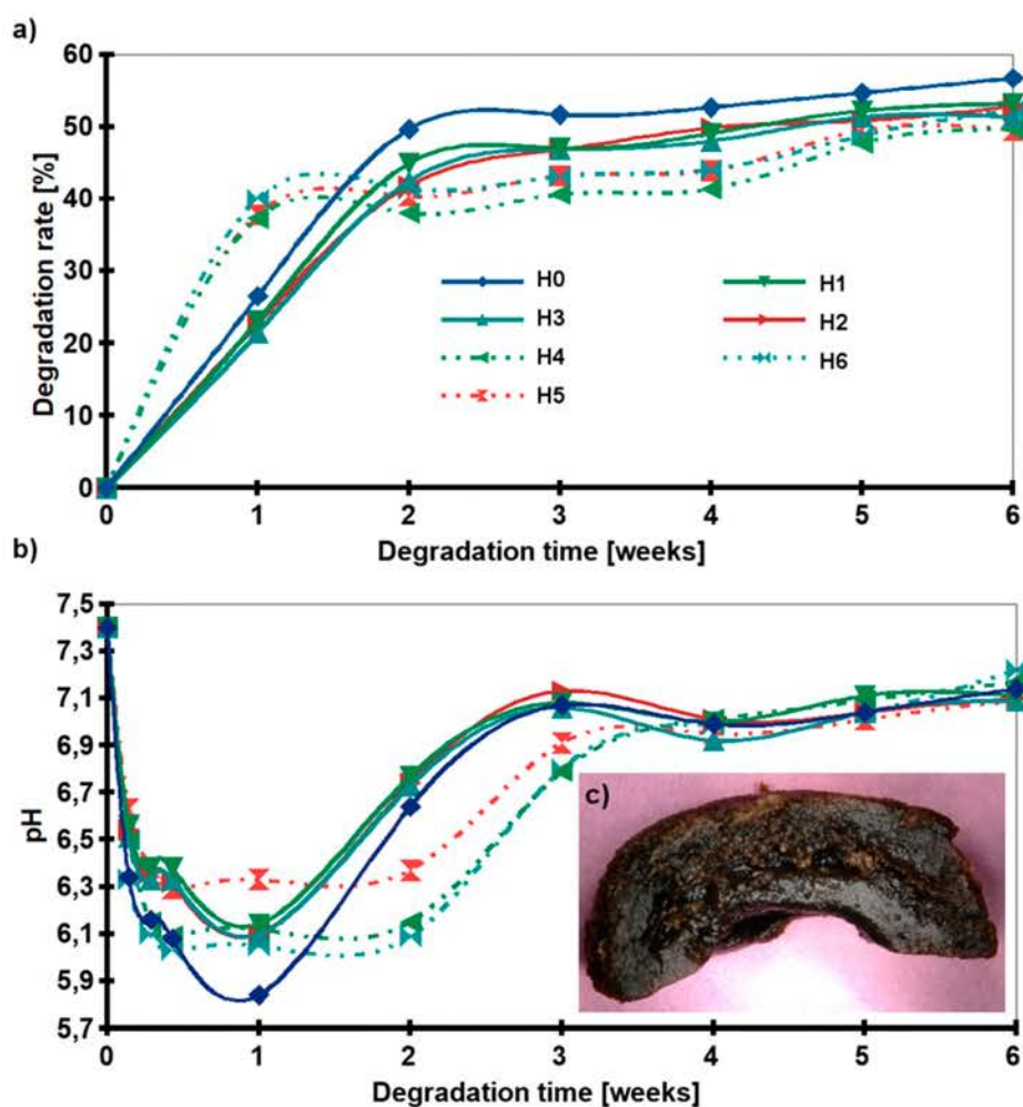
Figure 7. Degradation behavior: (a) Weight loss of the samples as a function of incubation time in PBS, (b) pH of media, (c) Digital microphotograph of H2 after 6 weeks of incubation (slice cut in half); (H0: chitosan (CS); H1: CS/graphene oxide (GO); H2: CS/poly(ethylene glycol) grafted graphene oxide (GO-PEG); H3: CS/reduced graphene oxide (rGO); H4: CS/GO/hydroxyapatite (HAp); H5: CS/GO-PEG/HAp; H6: CS/rGO/HAp).
