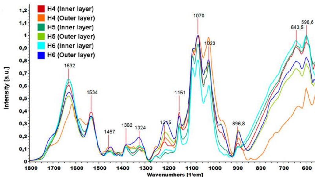
Figure 9. Parts of FTIR (Fourier transform infrared spectroscopy) spectra of hydrogels (H4: chitosan (CS)/graphene oxide (GO)/hydroxyapatite (HAp); H5: CS/ poly(ethylene glycol) grafted graphene oxide /HAp; H6: CS/reduced graphene oxide/HAp) in the range 1800–550 \text{cm}^{-1} .
