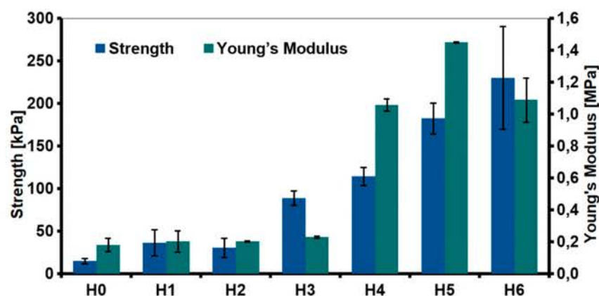
Figure 11. Mechanical properties (compressive strength and Young's modulus) of the hydrogels (H0: chitosan (CS); H1: CS/graphene oxide (GO); H2: CS/poly(ethylene glycol) grafted graphene oxide (GO-PEG); H3: CS/reduced graphene oxide (rGO); H4: CS/GO/hydroxyapatite (HAp); H5: CS/GO-PEG/HAp; H6: CS/rGO/HAp).
