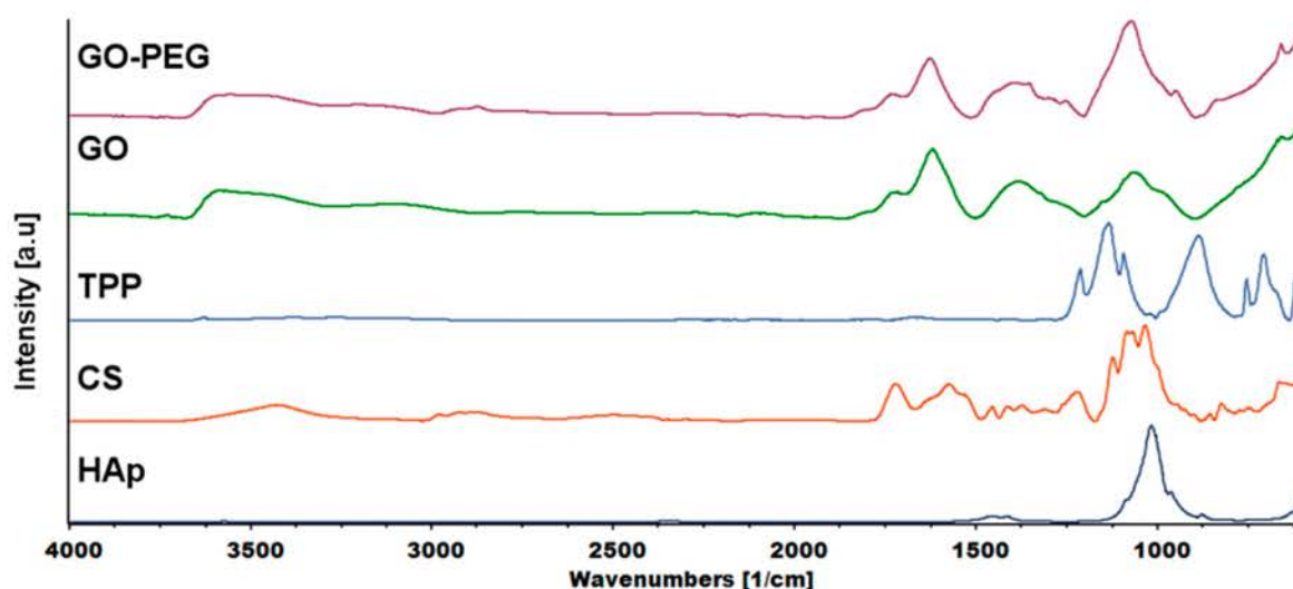
Figure 8. FTIR (Fourier transform infrared spectroscopy) spectra of the hydrogels components: HAp—hydroxyapatite, CS—chitosan, TPP—sodium tripolyphosphate, GO—graphene oxide, GO-PEG poly(ethylene glycol) grafted graphene oxide).
