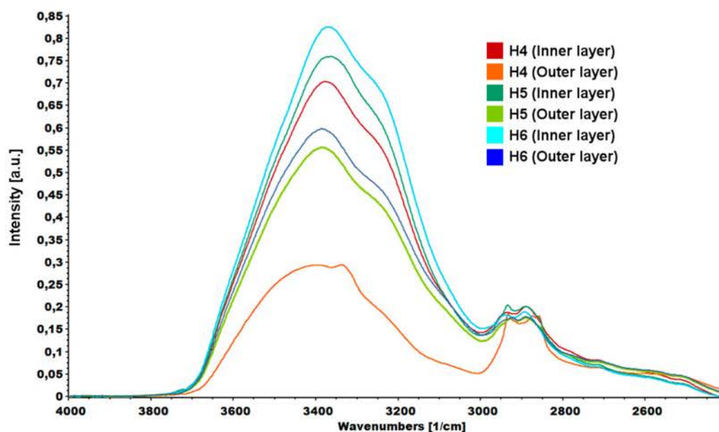
Figure 10. FTIR spectrum of hydrogels (H4: chitosan (CS)/graphene oxide (GO)/hydroxyapatite (HAp); H5: CS/ poly(ethylene glycol) grafted graphene oxide /HAp; H6: CS/reduced graphene oxide/HAp) peaks assigned to -\text{OH} vibrations.
