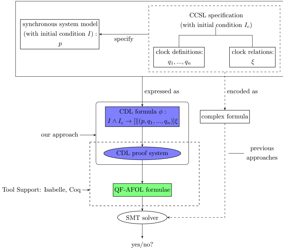
Figure 1: Verification framework of CDL
