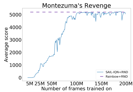
Figure 8: Combining SAIL and RND elevates the performance of IQN and matches that of RND-Rainbow, the best reported in Taiga et al. [42] on Montezuma's Revenge.
