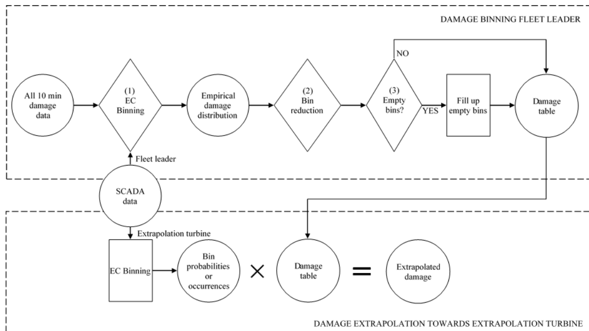
Figure 1: A simplified overview to extrapolate damage data from one turbine to another, with indication of several choices that are part of the procedure.
