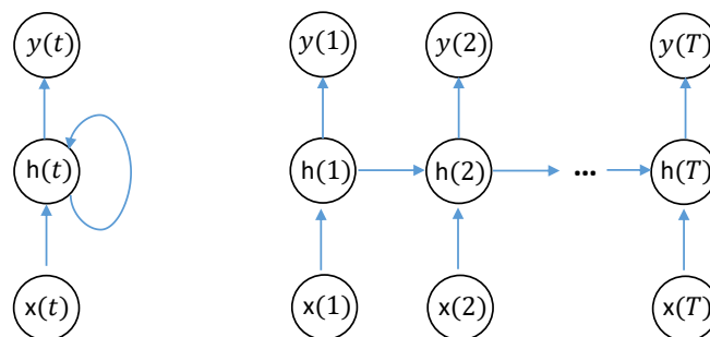
Figure 11. Graphical formulation of Recurrent Neural Networks.
