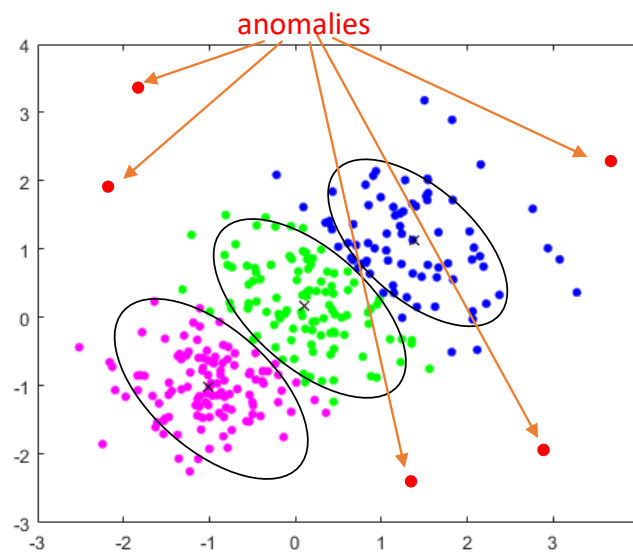
Figure 15. Illustration of anomaly detection.
