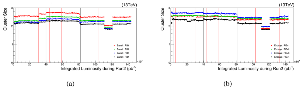
Figure 2. RPC cluster size vs integrated luminosity during RUN-2 for barrel in (a) and endcap in (b). Red vertical lines show the planned technical stops (TS) and the grey ones — Year-End-Technical stops (YETS).
