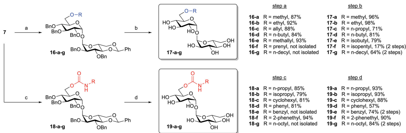
Scheme 2. Synthesis of 6- O -substituted trehalose derivatives. Reagents and conditions: (a) 2.5 eq NaH, 4 eq R-Br or R-I, DMF, 16 h; (b) 0.05 eq Pd/C, EtOAc/MeOH 1/1, 16 h; (c) 3 eq R-N=C=O, 0.2 eq DMAP, CH 2 Cl 2 , 24–120 h.
