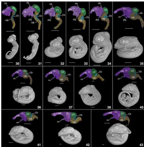
Figure 8. Embryonic development of the Lepidodactylus lugubris brain visualized through soft-tissue \mu CT. Whole-embryo \mu CT images are pictured below the corresponding isolated brain. The four distinct regions of the brain are color-coded as follows: telencephalon + diencephalon, purple; Optic tectum, green; Cerebellum, blue; Hindbrain, yellow. Scale bars = 1 mm. Cb, cerebellum; Cr, cerebrum; HB, hindbrain; OB, olfactory bulbs; ON, optic nerve; OT, optic tectum; pg, pineal gland; ptg, pituitary gland
