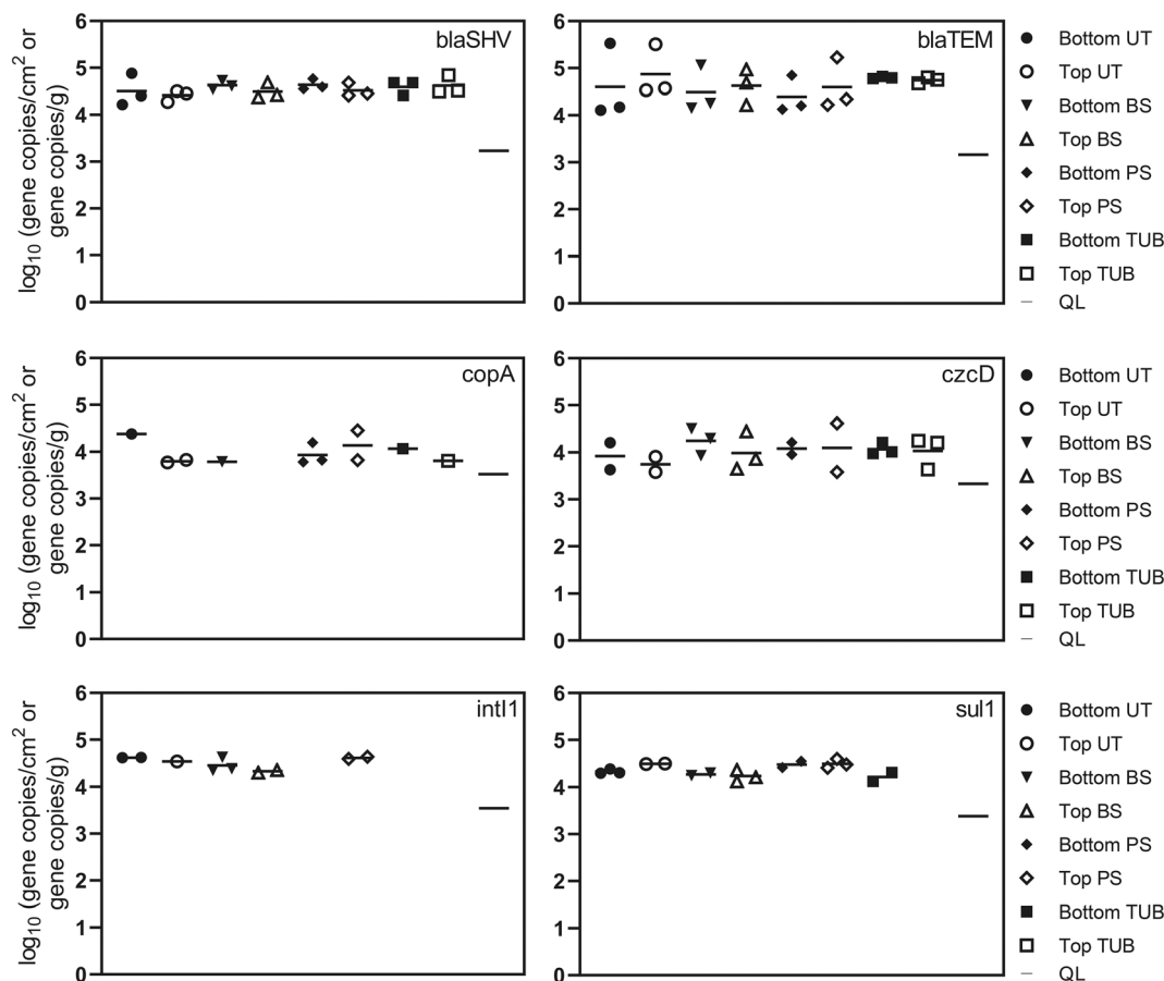
Fig. 2 Absolute abundance of antibiotic resistance genes, metal resistance genes, and int11 in different biofilm microenvironments from a cast iron drinking water main as measured with ddPCR. The biofilm microenvironments include biomass surface (BS), pipe surface (PS), tubercle (TUB), and under tubercle (UT). Each biofilm sample is also categorized by top or bottom pipe sample location. Sample categories (e.g. bottom UT, top BS) are plotted when 1–3 of the samples yielded a quantifiable result. Sample categories with no positive detections were left blank. Each symbol represents the average of 3 ddPCR technical replicates from a single biofilm sample. All biofilm swab samples are plotted as log 10 gene copies per cm 2 . Corrosion tubercle samples are plotted as log gene copies per g. The quantification limit (QL) is also plotted for each gene as the dash on the right side of the plot.
