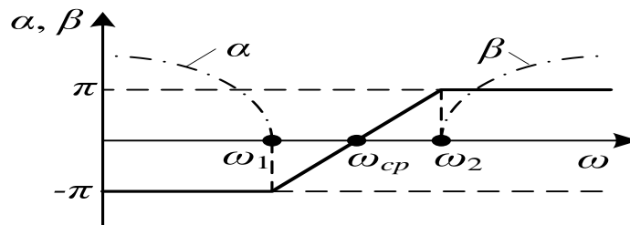
Figure 1. The structure damping ( \alpha –attenuation coefficient and \beta – coefficient of phase change) of the output signal in long electrical line is characterized by propagation constant: \alpha – attenuation coefficient of wave in the control line of US, characterizes the change amplitude of wave per unit length of the line; \beta – coefficient of phase change of an electrical signal in long control line of U (eq. 2 and 6).
