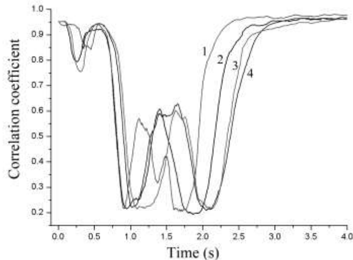
Figure 6. Time dependences of the correlation coefficient during the combustion of the mixture of aluminium and iron nanopowders.
