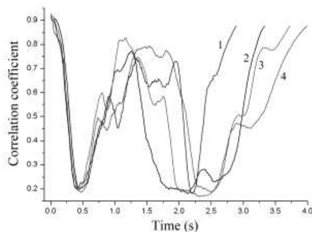
Figure 5. Time dependences of the correlation coefficient during the combustion of four aluminium nanopowder samples.
