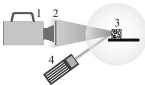
Figure 1. Experimental scheme: 1 – high-speed monochrome camera with objective, 2 – 532 nm narrow-band filter, 3 – cuboid nanopowder, 4 – Nd:YAG laser.
