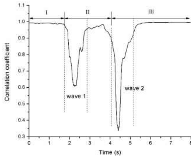
Figure 4. The schematic time dependence of the correlation coefficient during the aluminium nanopowder combustion.
