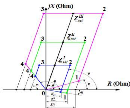
Figure 2. Distance protection polygonal characteristics.
