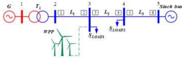
Figure 4. Experimental scheme with the installation of wind turbines at the end of the protected power line L_1 .
