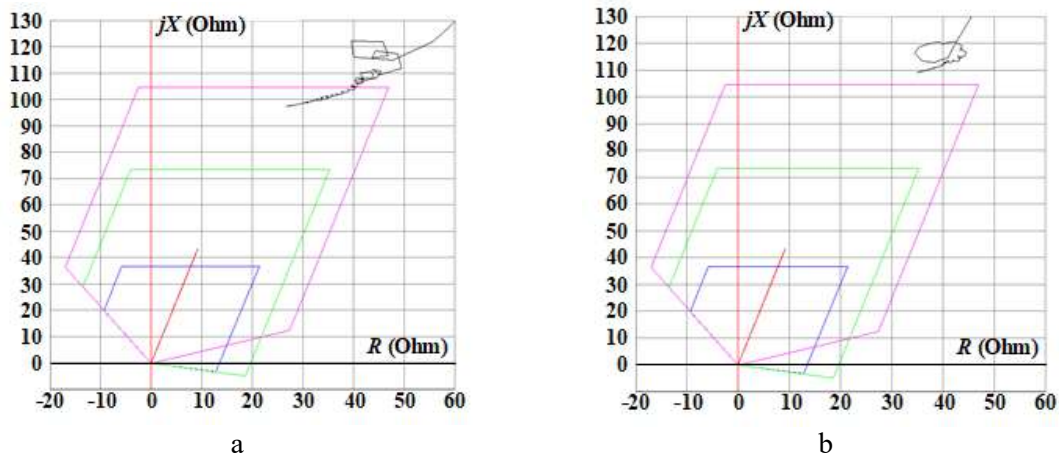
Figure 5. Hodograph of (a) the phase A impedance in case of a 3LG fault and (b) the impedance between phases A and B in case of a LL fault at the end of the adjacent line L_2 at wind speed of 18 \text{ km/h} = 5 \text{ m/s} .
