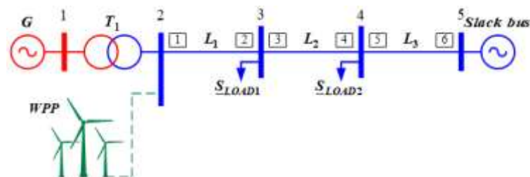
Figure 3. Experimental scheme with the installation of wind turbines at the beginning of the protected power line L_1 .
