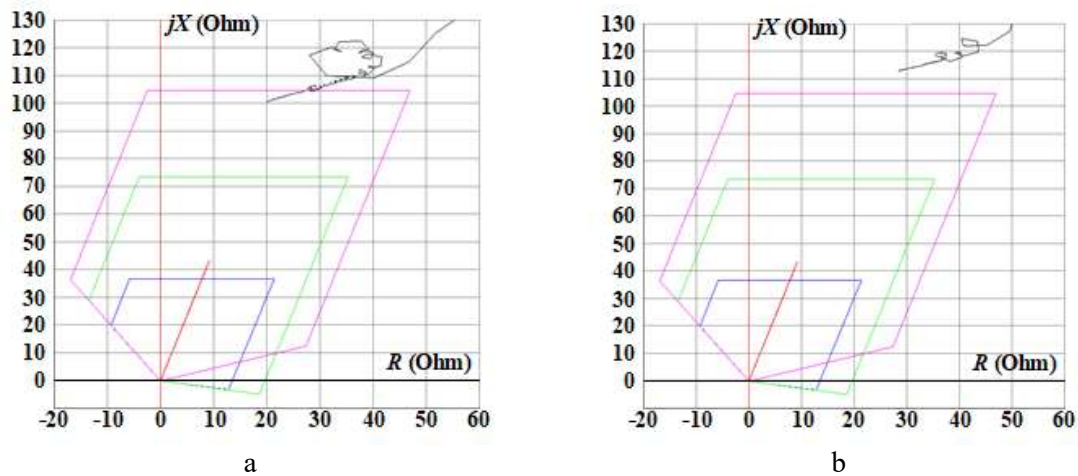
Figure 6. Hodograph of (a) the phase A impedance in case of a 3LG fault and (b) the impedance between phases A and B in case of a LL fault at the end of the adjacent line L_2 at wind speed of 36 \text{ km/h} = 10 \text{ m/s} .
