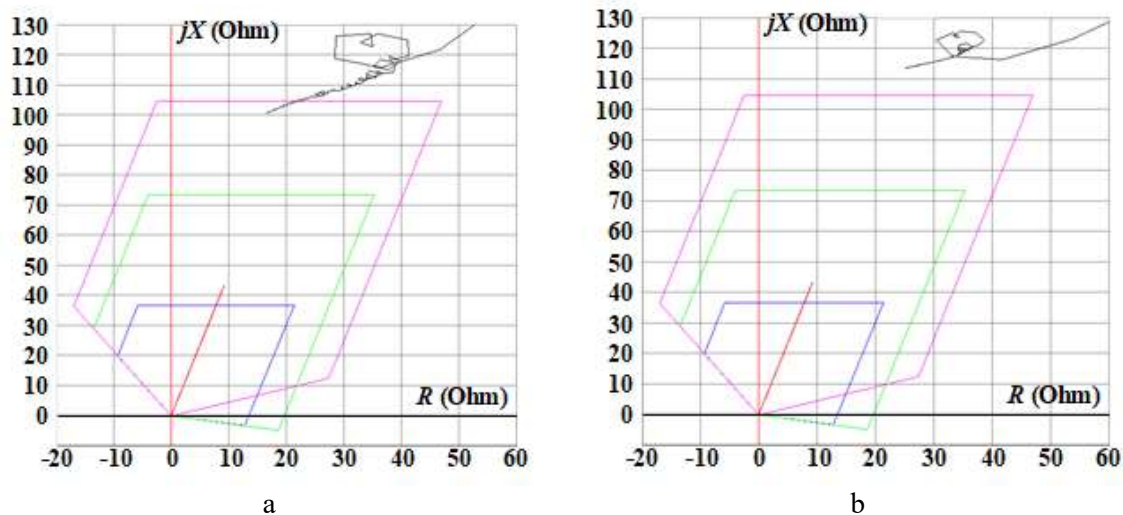
Figure 7. Hodograph of (a) the phase A impedance in case of a 3LG fault and (b) the impedance between phases A and B in case of a LL fault at the end of the adjacent line L_2 at wind speed of 50 \text{ km/h} \approx 14 \text{ m/s} .
