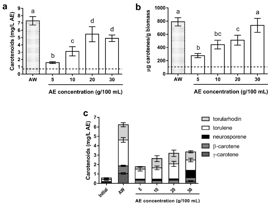
Fig. 5 Carotenoid production of Rh. mucilaginoso at different mediums. a Total carotenoid volumetric production; b specific carotenoid production. c Torularhodin, torulene, β-carotene and neurosporene contents obtained at mediums after 4 days of culture. Bars show the mean and S.D. ( n = 3 ), different letters indicate statistically significant differences ( p < 0.01 )
