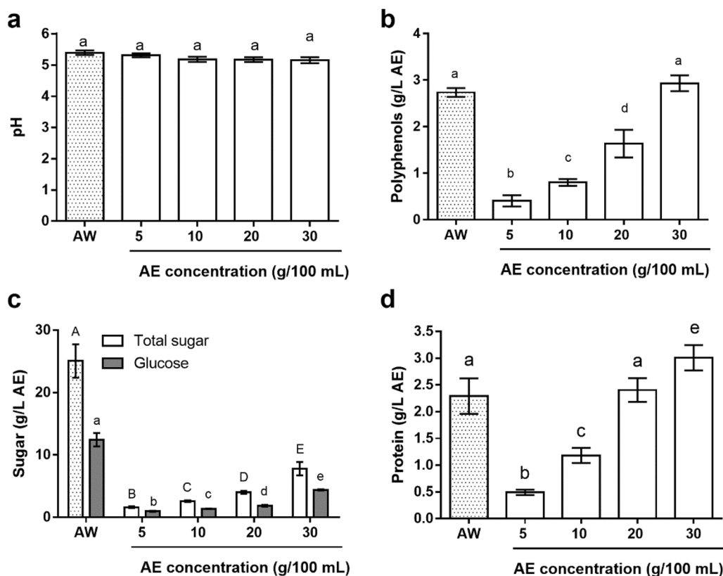
Fig. 1 Physicochemical characteristics of different media. pH (a), polyphenol content (b), Total sugar and glucose contents (c) and protein contents (d) were measured in the different media used as substrate for carotenoid production by Rh. mucilaginos a. Bars show the mean and S.D. values (n = 4); different letters indicate statistically significant differences (p < 0.01)
