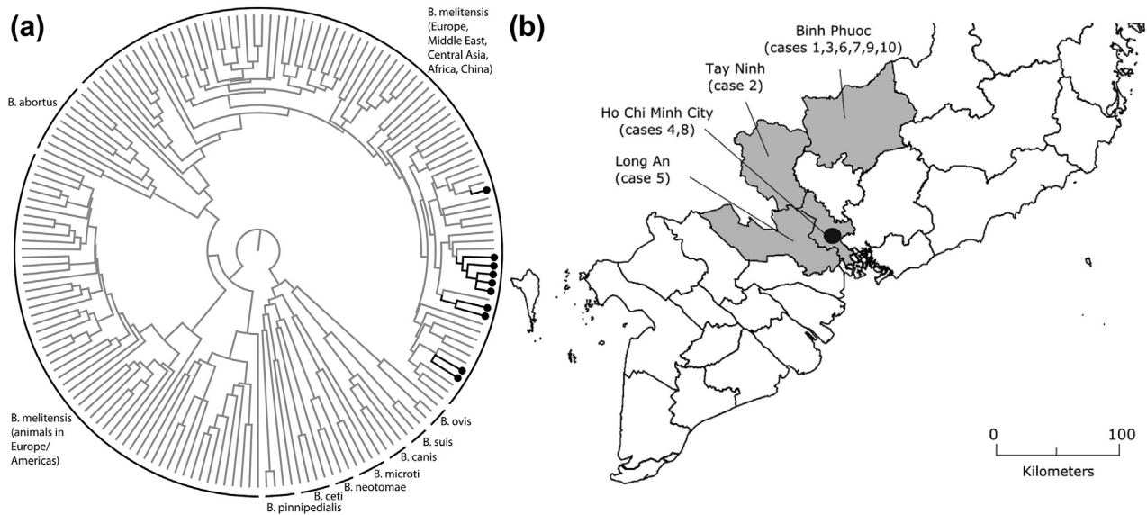
Fig. 1. Locations and MLVA genotypes of 10 human Brucella melitensis cases in southern Vietnam. (a) Circular tree representing the global population structure of the genus Brucella using Multiple Locus VNTR Analysis-16 (MLVA-16) analysis. Nine different Brucella species (labelled) are shown and associated with main branches; B. melitensis forms the majority of the tree. The 10 Vietnamese isolates are on black branches within the B. melitensis population. (b) Map of southern Vietnam showing the locations of provinces where the 10 cases of brucellosis originated between June 2016 and January 2017. The solid circle shows the location of the Hospital for Tropical Diseases in Ho Chi Minh City.
