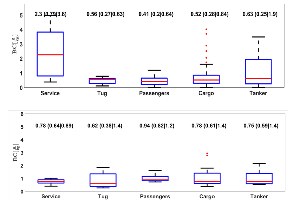
Figure 17. BC measurements in St Petersburg, Russia (upper panel) and Tricity, Poland (lower panel).
