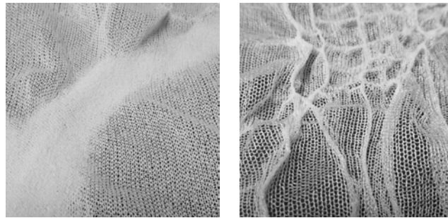
Figure 2: The textiles used and examples of modifications. Left: Trevira CS PEMOTEX ® , interlock knitted with 2 yarns. Right: COMFIL ® PET, single jersey knitted with 1 thread.
