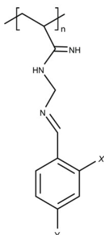
Figure 6. Polyacrylonitrilbenzaldehyde.
