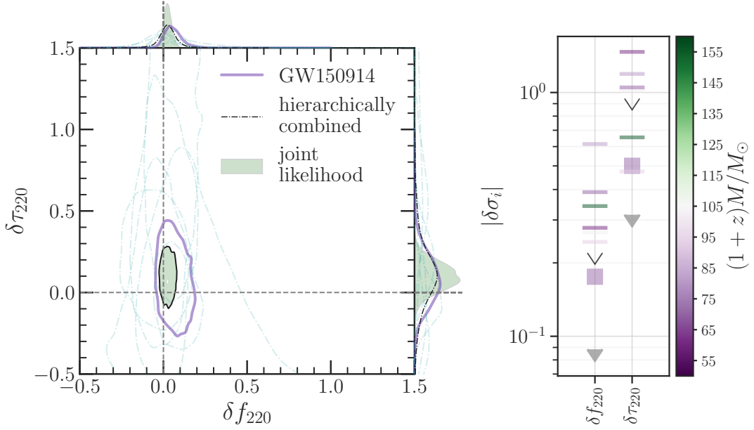
FIG. 6. Left panel : The 90% credible levels of the posterior probability distribution of the fractional deviations in the frequency and damping time of the (2, 2) QNM, (\delta f_{220}, \delta \tau_{220}) and their corresponding one-dimensional marginalized posterior distributions, for events from O1, O2 and O3a passing a SNR threshold of 8 in both the pre- and post-merger signal. The solid purple curve marks the best single-event constraint, GW150914, whereas the constraints from the other events are indicated by the dash-dot curves. The joint constraints on (\delta f_{220}, \delta \tau_{220}) obtained multiplying the likelihoods from individual events is given by the filled grey contours, while the hierarchical method of combination yields the black dot dashed curves. Right panel : 90% credible interval on the one-dimensional marginalised posteriors on \delta \sigma_i = (\delta f_{220}, \delta \tau_{220}) , colored by the median redshifted total mass (1+z)M , inferred assuming GR. Filled gray (unfilled black) triangles mark the constraints obtained when all the events are combined by multiplying likelihoods (hierarchically). The purple square marker indicates constraints from the single most-prominent event, GW150914.
