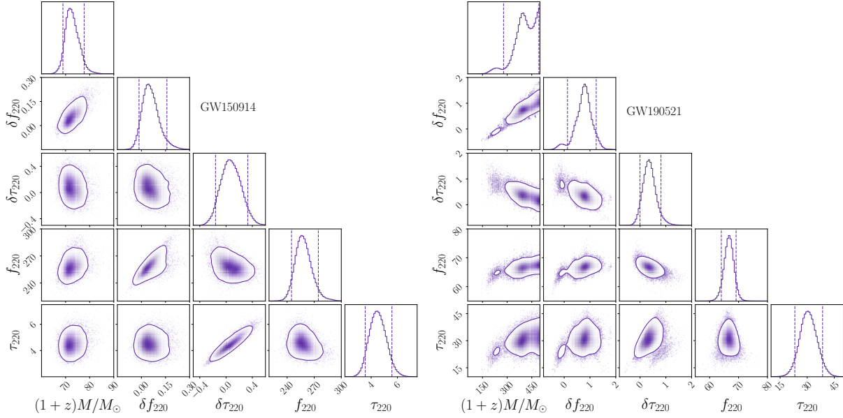
FIG. 8. Corner plots showing the correlations between the detector-frame total (1+z)M , the non-GR deviations ( \delta f_{220} , \delta\tau_{220} ) and the reconstructed frequency and damping time ( f_{220} , \tau_{220} ). The left panel shows results for GW150914, for which \text{SNR} > 8 in both the pre- and post-merger phase of the signal, and the correlations are absent. The right panel shows the results for GW190521, which has \text{SNR} > 8 in the post-merger phase, but not in the pre-merger phase, and the correlations are present.
