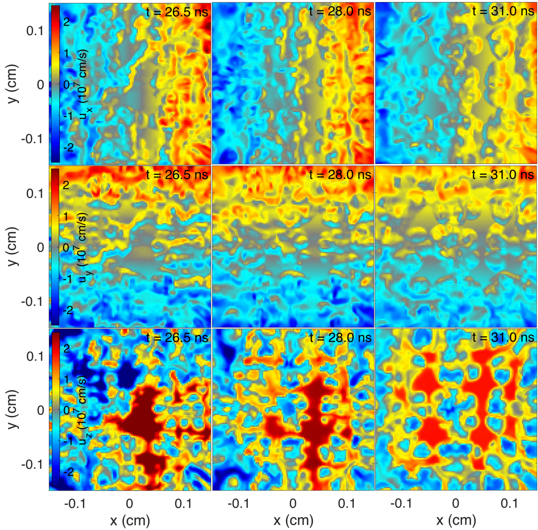
Fig. S19. Perpendicular slices of the velocity field in the FLASH simulations. Pseudo-color two-dimensional slices plots [in the (x, y) plane] of the three components of velocity in the FLASH simulations at t = 26.5 ns (left column), t = 28.0 ns (middle column) and t = 31.0 ns (right column). The slices are taken at the position on the z axis coincident with the lineouts shown in Figure S18.
