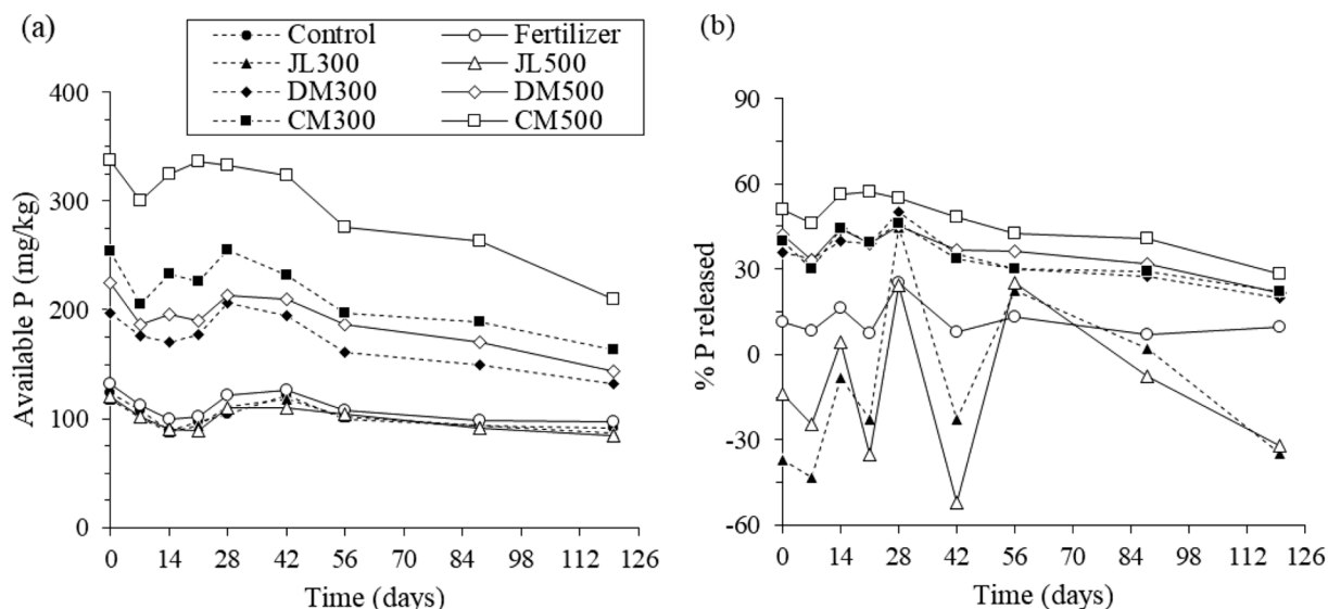
Fig. 3. Effect of fertilizer and biochar treatments on a) phosphorus availability and b) % phosphorus released.
