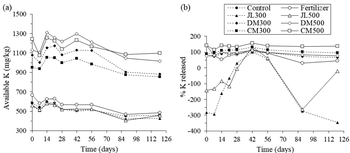
Fig. 4. Effect of fertilizer and biochar treatments on a) potassium availability and b) % potassium released.
