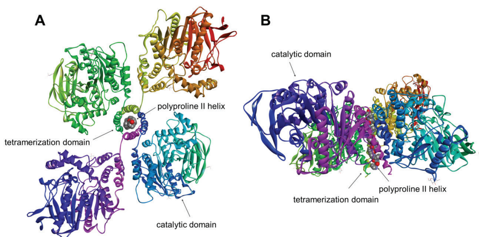
Figure 1. Cryo-EM structure of the native BChE tetramer (PDB 6I2T). A) Top view of the BChE tetramer as dimer of dimers in which the monomers are diagonally equivalent with polyproline II helix in the centre. B) Side view of the BChE tetramer with tetramerization domain concealed between dimers.
