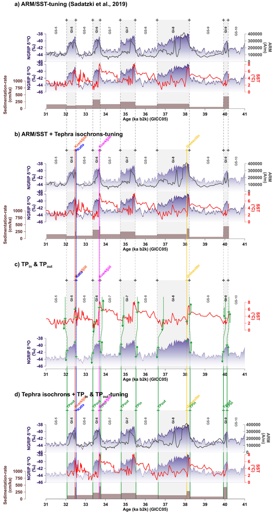
Fig. 9. Tephra-based synchronization and age model refinement of MD99-2284. For panel a, b and d, both ARM (dark grey) and SST (red) of MD99-2284 (Dokken et al., 2013) are plotted on top of NGRIP \delta^{18}O (purple) (Andersen et al., 2004, 2006; Seierstad et al., 2014). In addition, for each step in the age model refinement (panel a, b and d), the
