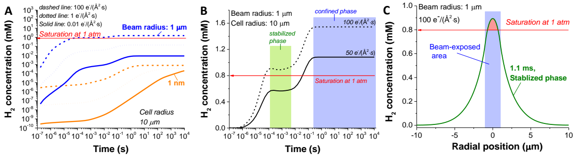
Figure 3 Influence of dose rate for small (1 nm) and large (1 μm) electron beam on H 2 concentration. (A) Temporal concentration profiles with various dose rates for the beam radius of 1 nm and 1 μm. (B) Profile comparison for 1 μm beam radius at two different electron dose rates: 50 and 100 e - /(Å 2 · s). (C) Spatial profile for 1 μm beam radius at 100 e - /(Å 2 · s).
