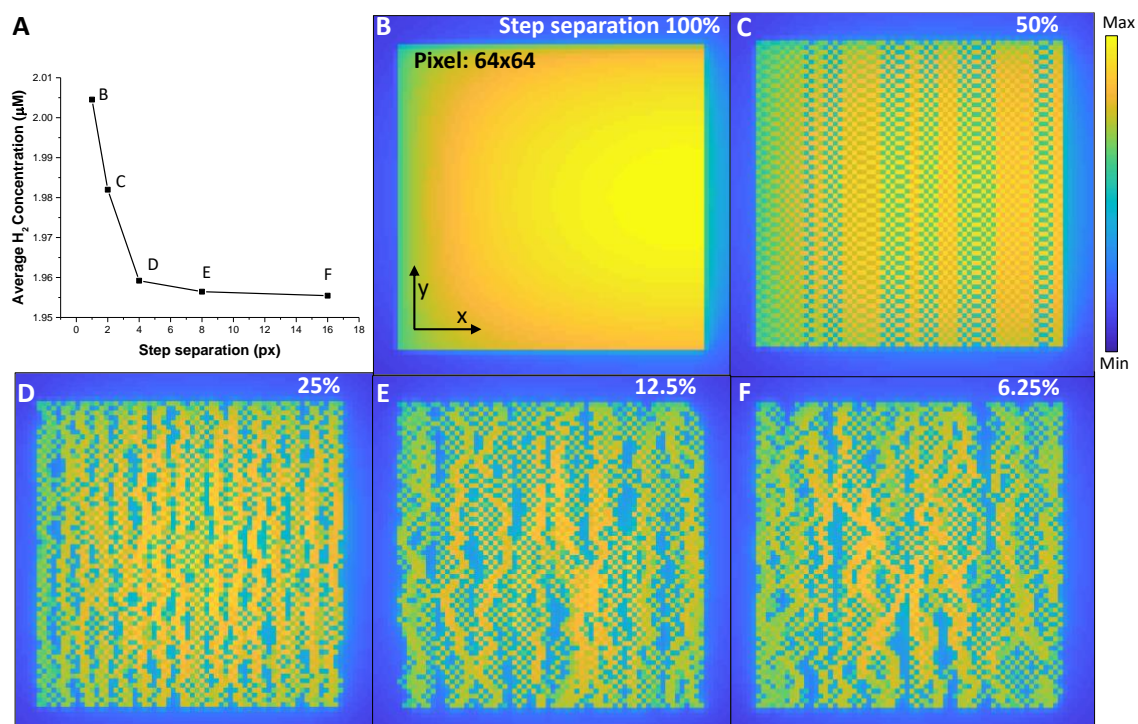
Figure 5: (a) the average H 2 concentration produced from a series of scans obtained with a step separation of 1 pixel (B), 2 pixels (C), 4 pixels (D), 8 pixels (E) and 16 pixels (F). For all scans the total beam dose and dose rate was kept constant with the only difference being the spatio-temporal profile of the beam delivery, i.e. the separation in space and time of the electrons hitting the liquid cell.
