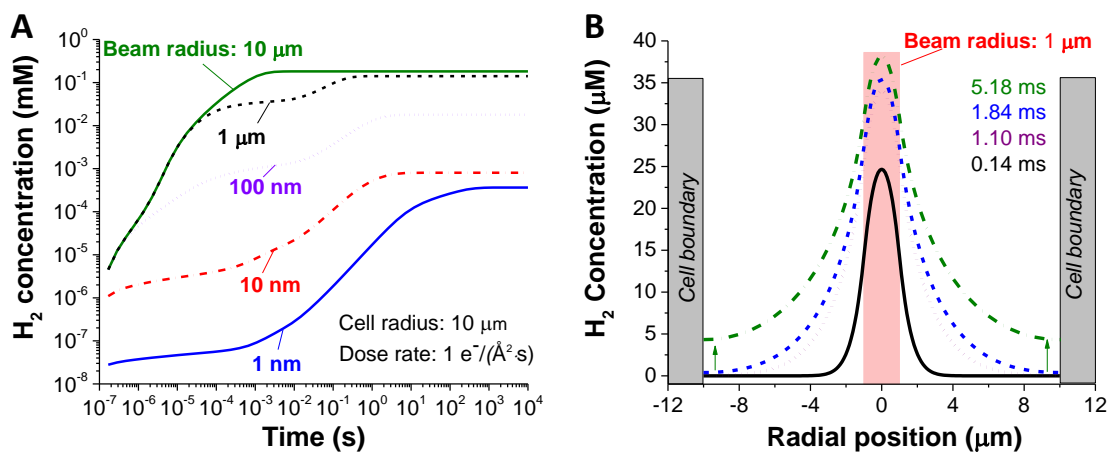
Figure 2 Concentration profiles of H_2 evolution during irradiation at an electron beam dose rate of 1 e^-/(\text{\AA}^2 \cdot s) . (A) Temporal profiles for increasing beam sizes in a cell radius of 10 \mu\text{m} . The initial onset of H_2 production quickly saturates for the beam that is the same size as the cell, whereas for the other beam sizes there are two plateaus. The first plateau appears while H_2 has not been reached to the cell boundary. After H_2 reaches the cell boundary, the concentration surges as the further diffusion is physically hindered. The second plateau occurs as a result of equilibrium. (B) Spatial profiles for the 1 \mu\text{m} beam at different irradiation times, showing the rise in concentration that is caused by the diffusion hindrance at the cell walls.
