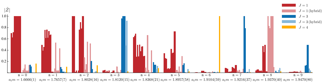
Figure 4. Normalised operator overlaps |\tilde{Z}| for the lowest 10 states in the T_1^{--} irrep on the 20^3 volume. The overlaps are normalised so that the largest value across all states is unity. Each state is labelled by its mass in lattice units determined in a variational analysis. The colours represent the continuum spin from which the operator was subduced and lighter colours indicate hybrid-like operators.
