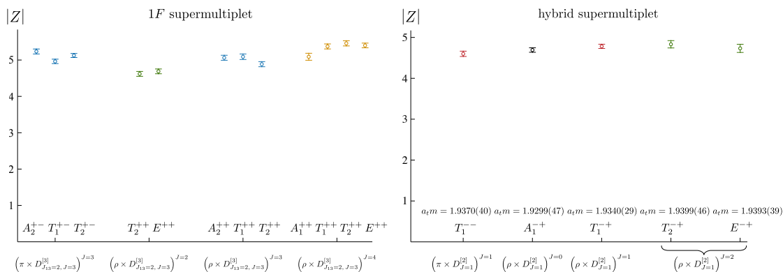
Figure 8. Operator overlap values |Z| for continuum operators corresponding to a 1F supermultiplet (left) and similarly a gluonic hybrid construction (right). These are subdivided into different irreps as indicated, with a consistent value found for the operator overlap across irreps.
