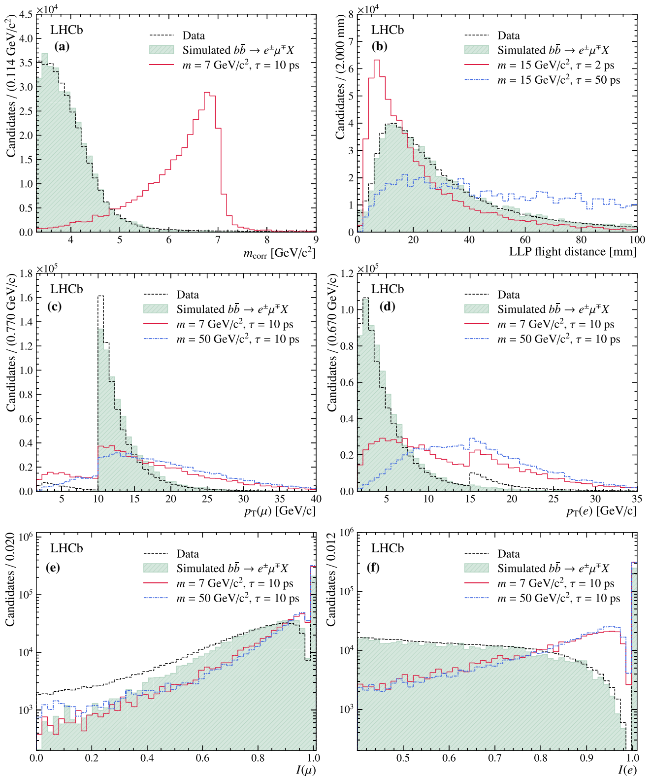
Fig. 2 Distributions in data (dashed black histogram) compared to simulated b\bar{b} \rightarrow e^\pm\mu^\mp X (green filled histogram), showing, a m_{corr} , b the LLP flight distance, c the transverse momentum of the muon, d the transverse momentum of the electron, e the isolation of the muon, and f the isolation of the electron. LLP signal distributions are also shown (coloured histograms) for different m_{LLP} and \tau_{LLP} values, where the
