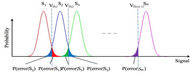
FIGURE 15: Gaussian probability density functions of multilevel signals.
