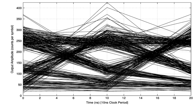
(b) Experimental eye diagram taken from [29].
