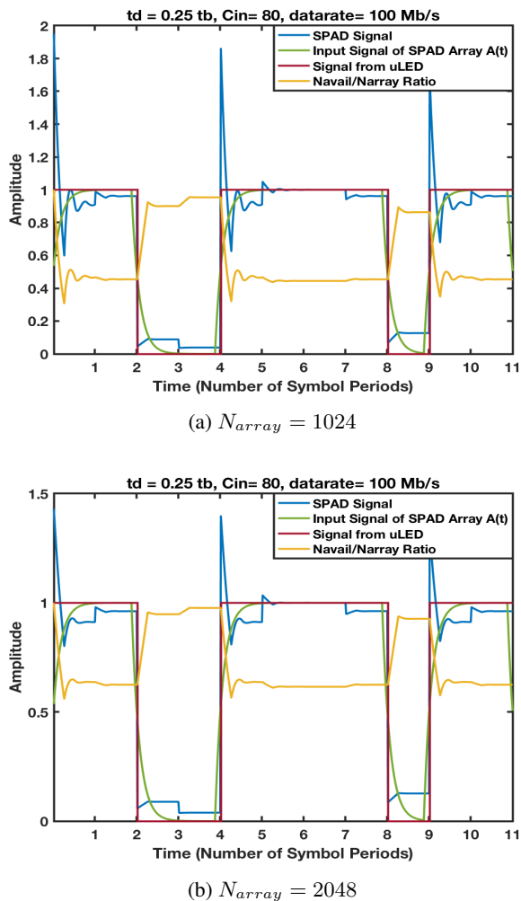
FIGURE 6: The demonstration of ISI using two examples N_{array} = 1024 for (a) and N_{array} = 2048 for (b) respectively, all simulations are with same parameters: 100 Mb/s, f_{RO} = 6.4 \text{ GHz} , PDE0 = 1 , P_{ap} = 0 , FF = 1 , DCR = 0 \text{ Hz/SPAD} , \tau_d = 16 \times T_I , C_a(n) = 80 , oversampling = 64 , \tau_d = 0.25T .
