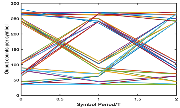
(a) Simulation eye diagram.
