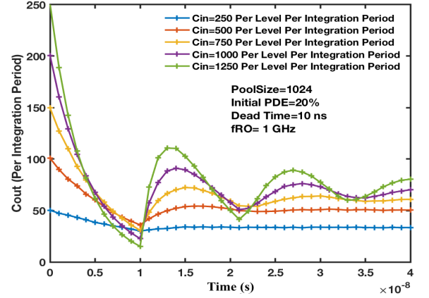
FIGURE 16: SPADs-based array signal nonlinearity. A modelled step response for SPAD-based receivers with increasing received photons counts.
