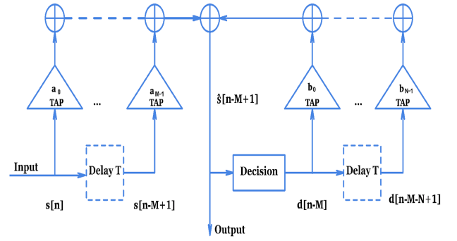
FIGURE 11: Schematic of combined FFE and DFE. The delay between each tap is T .
