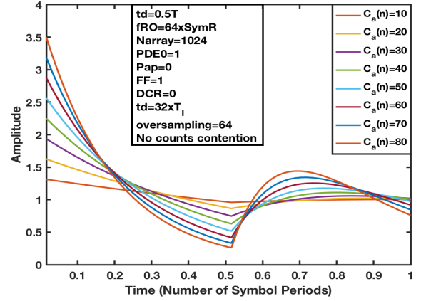
FIGURE 3: Modelled normalised step response with a sweep of C_a(n) . C_a(n) is the average received number of photons per normalised signal power per integration period. The parameters used are described in the figure.
