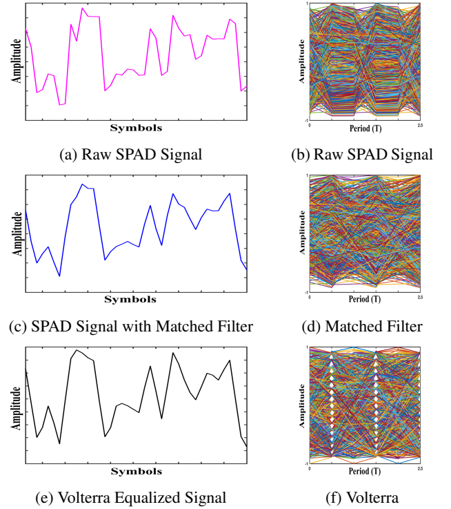
FIGURE 14: 1 Gbit/s high received optical power PAM-16 back-to-back link with Volterra equalisation. Simulation parameters are: readout frequency f_{RO} = 500 MHz, dead time = 2 ns, symbol rate = 250 Mbaud, 1000 symbols, N_{array} = 1024 , PDE0 = 1 , P_{ap} = 0.01 , FF = 1 , DCR = 2.5 \times 10^3 per SPAD, FFE taps = DFE taps = 2, FFE tap spacing = symbol spaced, adaptation loops = 20.
