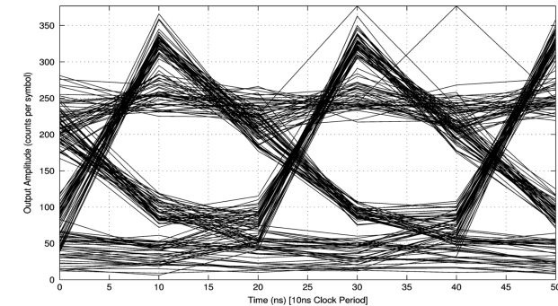
(b) Experimental eye diagram taken from [29].
