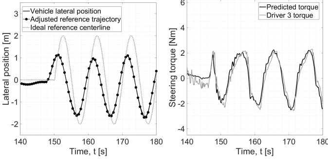
Fig. 4. Driver model predictions based on driver 3, expert level
