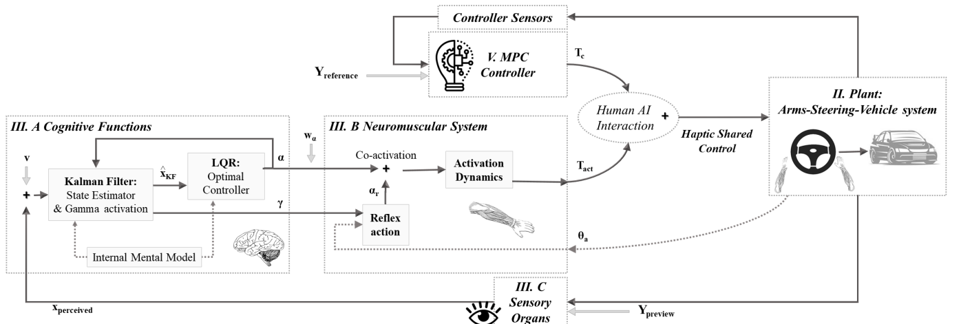
Fig. 2. Haptic Shared Control scheme with driver model representation. A detailed description of each block can be found in the corresponding sections.
