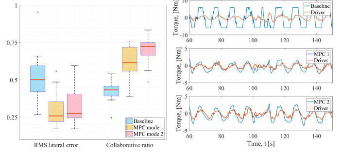
Fig. 8. (a) Box plot of the objective KPIs of 19 participants (b) Torques over time for participant 1.
