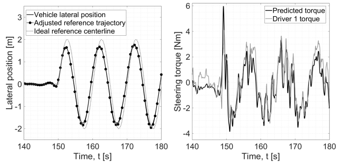
Fig. 3. Driver model predictions based on driver 1, novice
