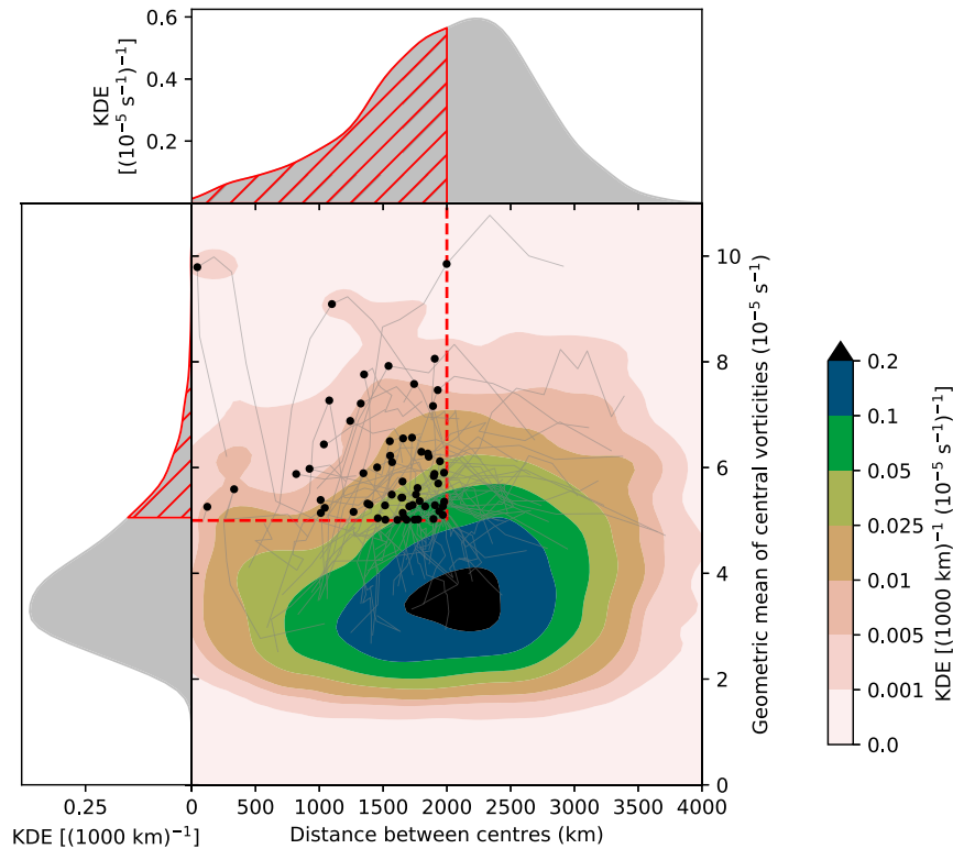
FIG. 1. Case studies shown in distance–intensity phase space. The selection thresholds [\sqrt{\zeta_{350}(\text{WD})\zeta_{850}(\text{TD})} > 5 \times 10^{-5} \text{ s}^{-1} and separation distance of the TD and WD centers < 2000 \text{ km} ] are marked in red. Paths of the 59 cases meeting these criteria are given by gray lines, with exemplary points for each marked in black. Colored contours show a Gaussian kernel density estimate of the frequency of all interactions (on a time step, rather than event, basis). The univariate Gaussian kernel density estimates for (top) distance and (left) intensity.
