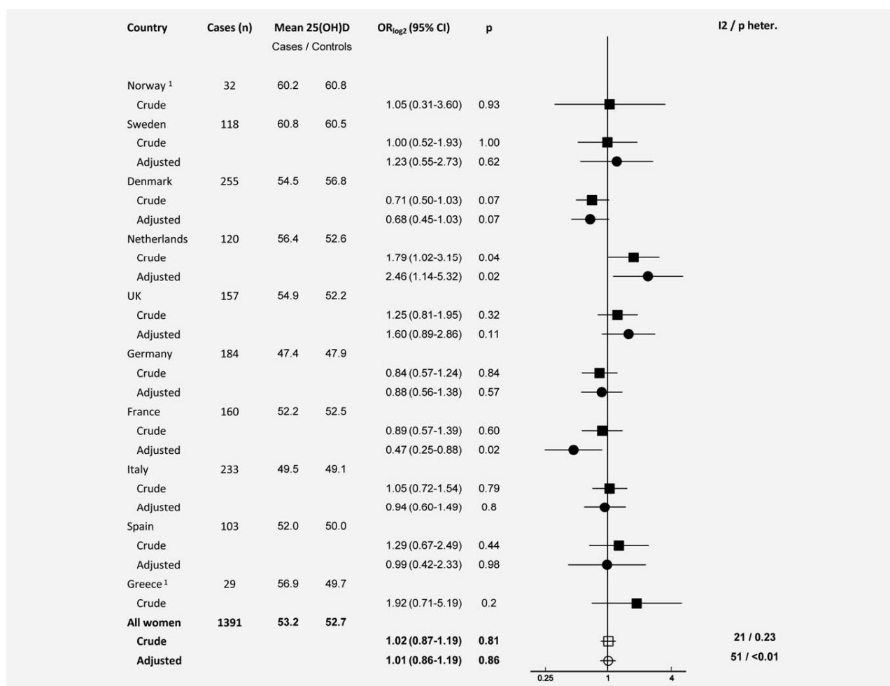
Figure 3. Country-specific odds ratios (95% CIs) of breast cancer according to season-standardized 25(OH)D levels on the log 2 scale. OR: odds ratio; CI: confidence interval; p heter.: p for heterogeneity. Results from conditional logistic regression matched for study center, age at blood donation, menopausal status, exogenous hormone use at blood donation, time of the day of blood collection, fasting status and phase of menstrual cycle (crude model) with additional adjustment for BMI, age at first period, age at first full-term pregnancy, number of full-term pregnancies, breastfeeding, alcohol consumption, smoking status, education level and physical activity (adjusted model). 1 Results from unadjusted models only are reported for Greece and Norway, as multiple adjustment was restricted because of the low case numbers from these countries.
