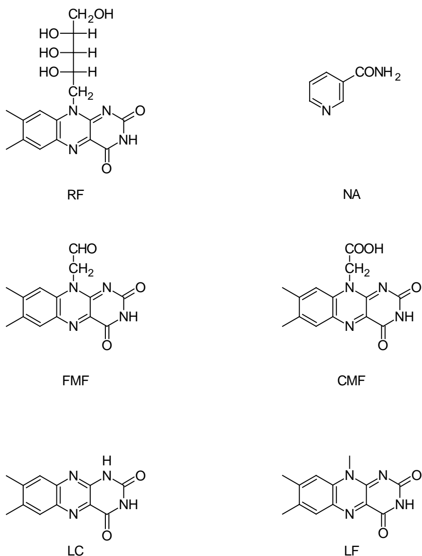
Fig. 1. Chemical structures of RF, its photoproducts (FMF, LC, LF, CMF) and NA.
