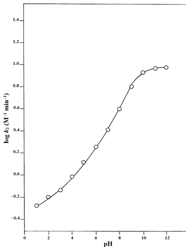
Fig. 3. \log k_2 –pH profile for the photolysis of RF in presence of NA.
