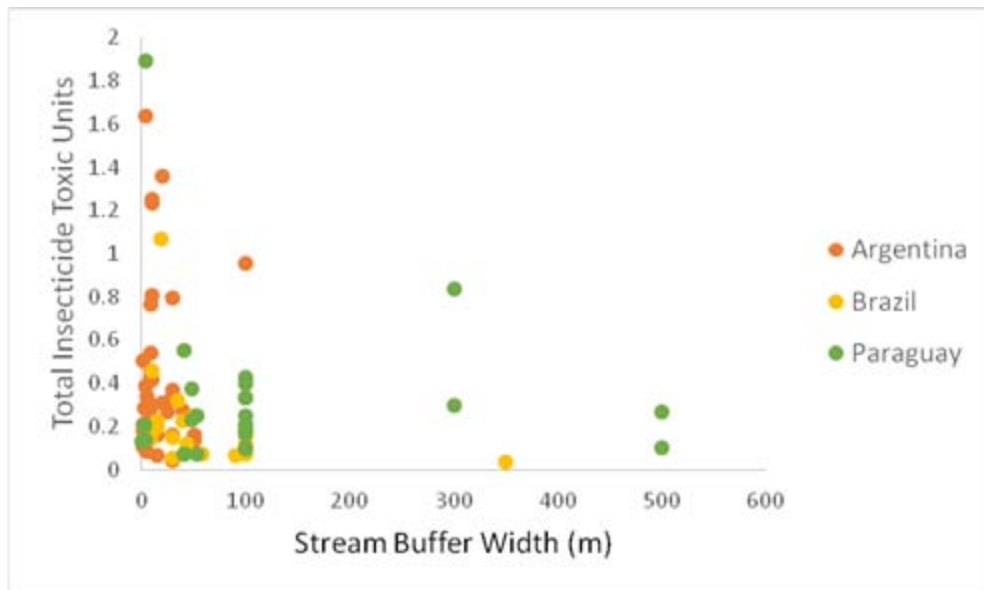
Figure 2. Relationship between riparian buffer width and total insecticide toxic units for all sites in the three intensive soy production regions studied in Brazil, Paraguay, and Argentina.
