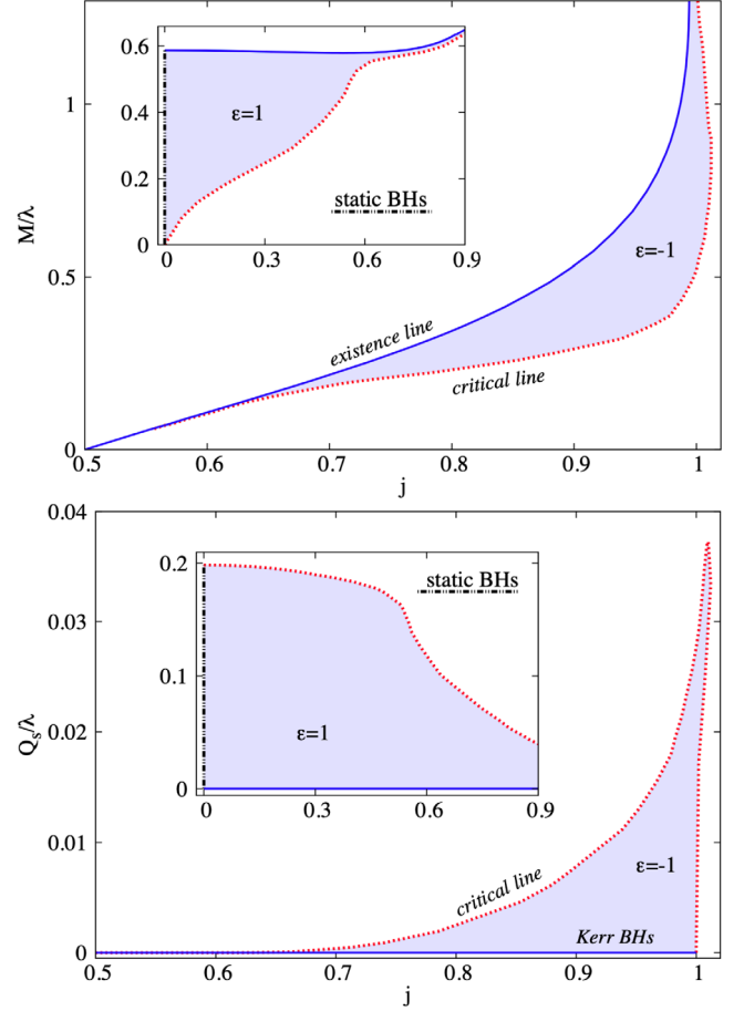
FIG. 1. ADM mass M (top panel) and scalar charge Q_s (bottom panel), both in units of \lambda , as functions of the dimensionless spin j of spinning scalarized BHs. Here and in Fig. 2, the main panels (insets) correspond to \epsilon = -1 ( \epsilon = +1 ).
