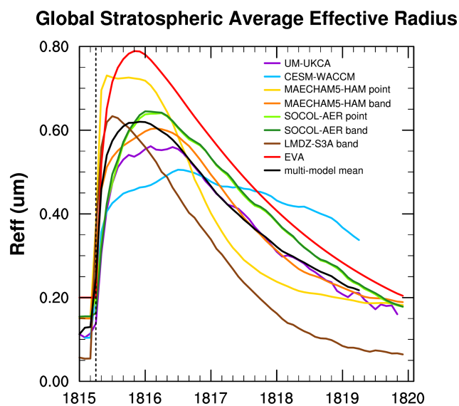
Figure 3. Global stratospheric mean effective radius ( R_{\text{eff}} ) time series. Vertical dotted line marks date of injection of SO 2 . The calculation of R_{\text{eff}} is weighted by surface aerosol density and grid cell volume, as explained in Appendix A.
