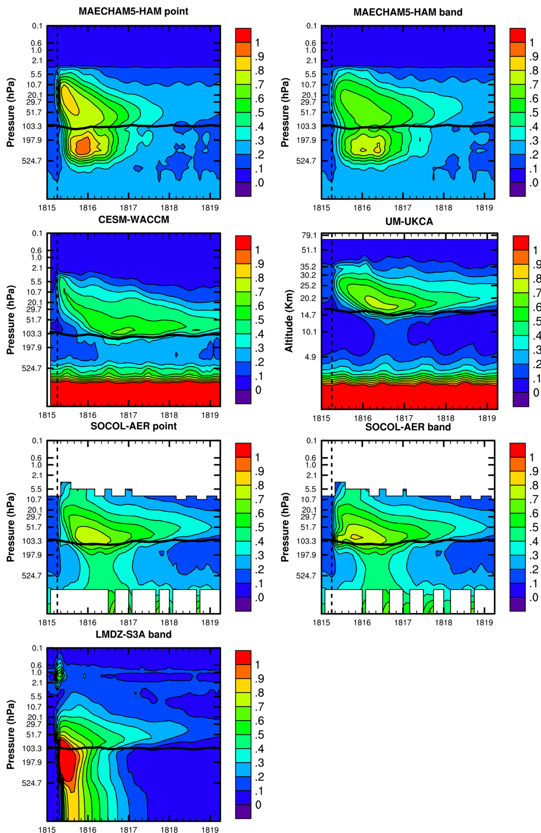
Figure 4. Vertical profile of tropical mean [23^{\circ}\text{S}, 23^{\circ}\text{N}] effective radius contours in units of micrometers ( \mu\text{m} ) marked by the color bar. A vertical dashed line marks the April 1815 injection. A horizontal solid black line marks tropopause height. The large particles in the lower troposphere in this figure (CESM-WACCM and UM-UKCA) are due to background particles such as sea spray and dust.
