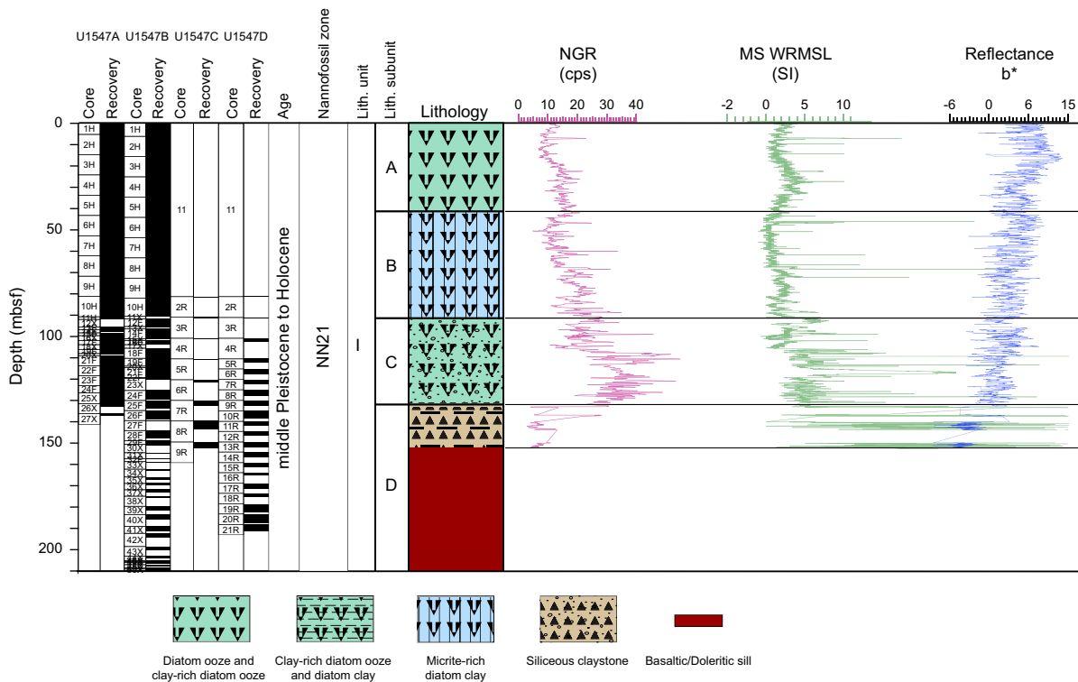
Figure F8. Lithostratigraphic column, Site U1547. NGR = natural gamma radiation, cps = counts per second, MS = magnetic susceptibility, WRMSL = Whole-Round Multisensor Logger. Reflectance b*.
