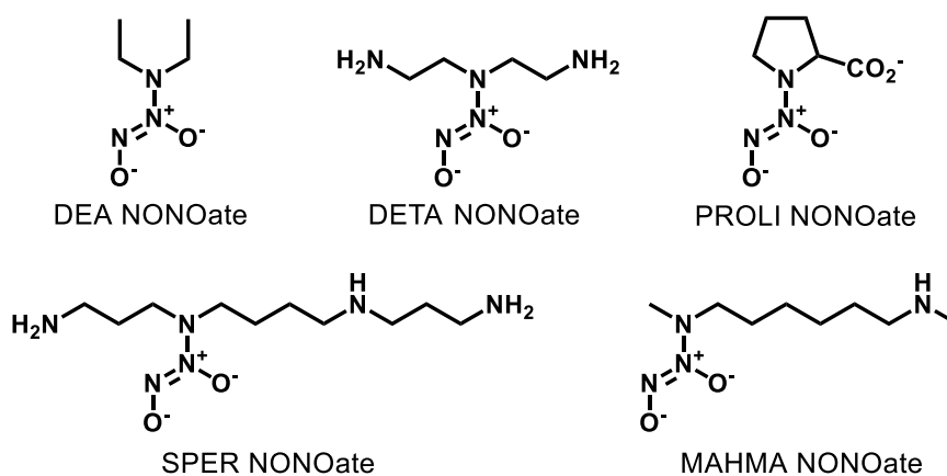
Figure 17. Structures of some NONOates derivatives molecules.
