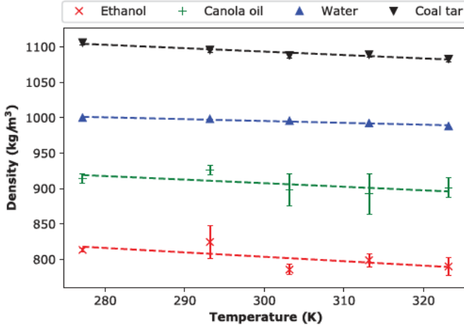
Fig. 1. Changes in canola oil, salty ethanol, water, and coal tar densities between 277.15 K and 323.15 K.
