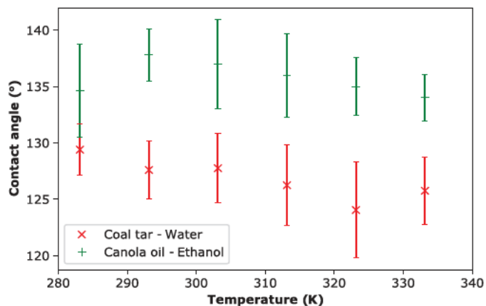
Fig. 4. Evolution of coal tar/water and canola oil/ethanol contact angle on a glass slide.
