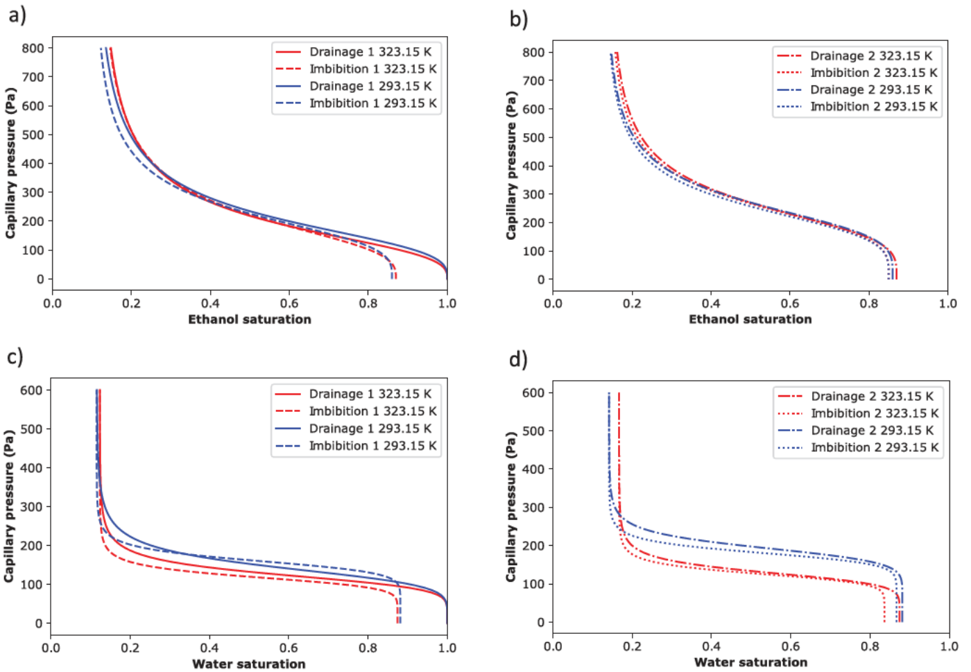
Fig. 8. Effect of temperature on capillary pressure-saturation curves for a) oil/ethanol primary curves, b) oil/ethanol main curves, c) coal tar/water primary curves, d) coal tar/water main curves.
