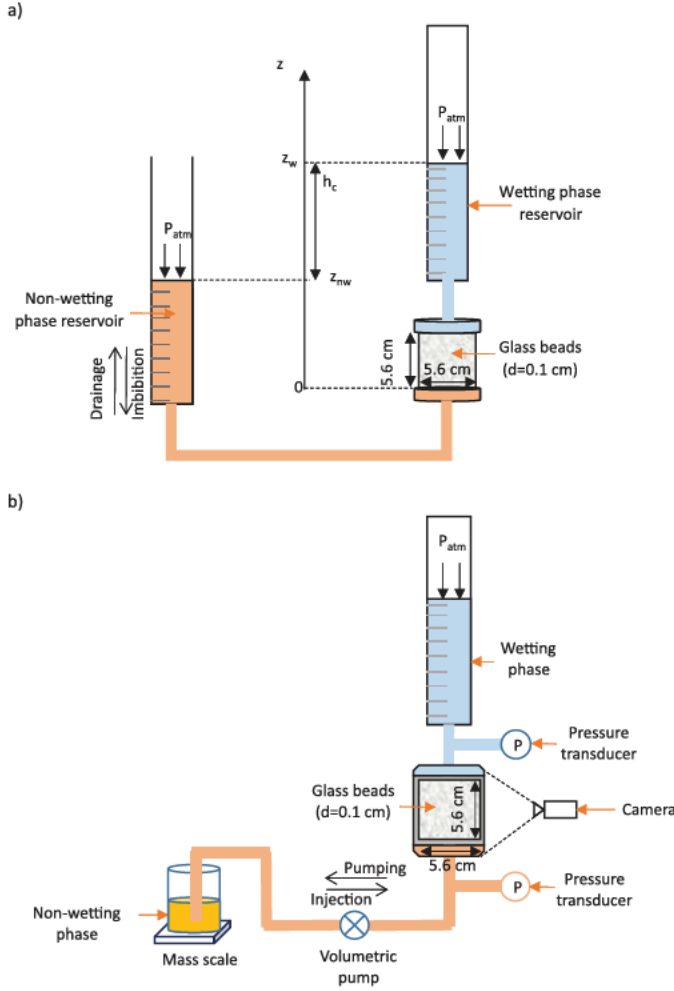
Fig. 5. Drainage/Imbibition setups used for (a) capillary pressure-saturation measurements and (b) setup used for experiments in dynamic conditions.
