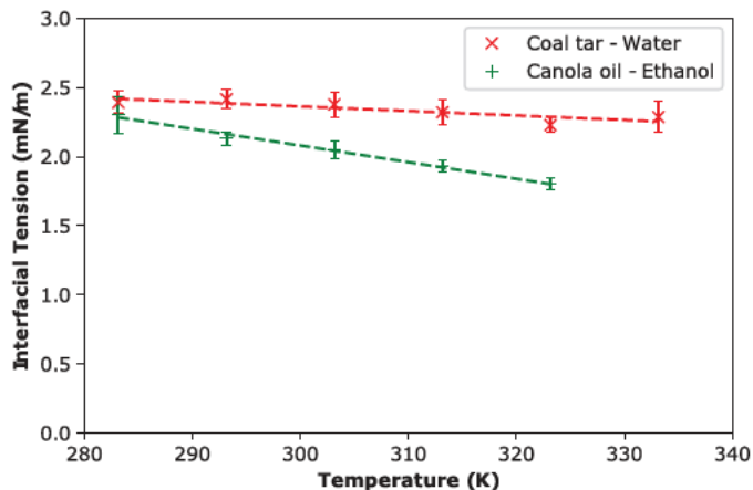
Fig. 3. Interfacial tension of canola oil/ethanol and coal tar/water as a function of temperature.
