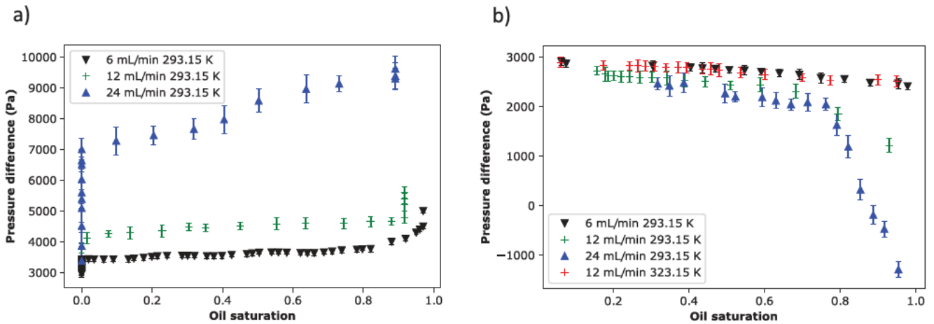
Fig. 10. Measured pressure difference during injection (a) and pumping (b) of oil.
