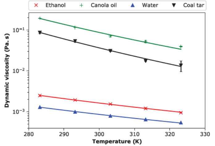
Fig. 2. Dynamic viscosity of salty ethanol, canola oil, water, and coal tar as a function of temperature. Lines represent data fitting with Andrade two-parameter exponential function.
