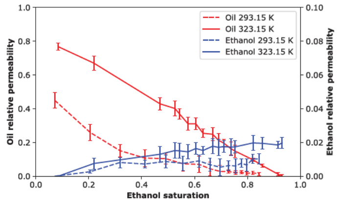
Fig. 11. Oil and ethanol relative permeabilities estimated during pumping at 12 mL/min at 293.15 K and 323.15 K.
