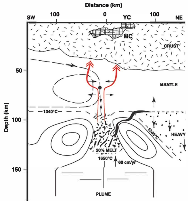
Figure 10. Schematic cartoon along an SW–NE cross-section of the subcontinental structures below YC according to our modelling of the plume and of the destabilization of the Wyoming lithosphere. MC: Magma Chamber whose geometry corresponds to the -2 per cent change of the P -wave velocity contour modified from Farrell et al. (2014), red arrows indicate the magma flow trajectories (see the text for details).
