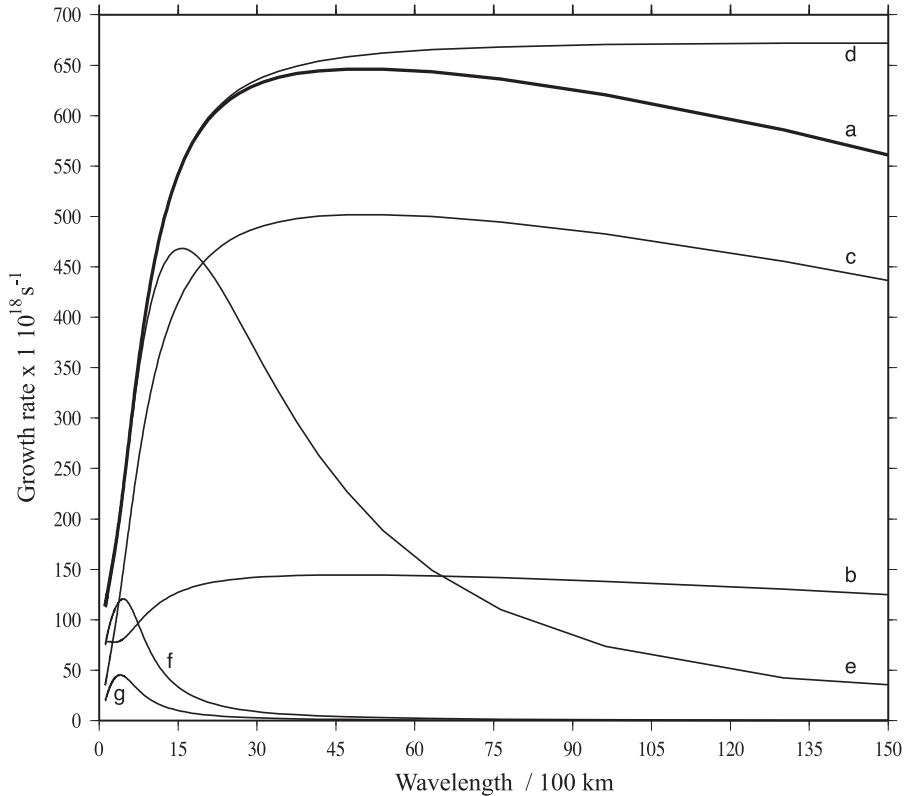
Figure 6. Instability analysis for n = 3 , that is, the lithosphere deforming by plastic creep. (a) reference curve where \eta_1 = 5 \times 10^{22} Pa s, \eta_2 = 10^{18} Pa s, \gamma = 10^{-16} \text{ s}^{-1} , \Delta\rho = 1 per cent; (b) idem as (a) but \Delta\rho = 0 per cent; (c) idem as (a) but \gamma = 0 ; (d) idem as (a) but \eta_2 = 10^{16} Pa s; (e) idem as (a) but \eta_2 = 10^{20} Pa s; (f) idem as (a) but \eta_2 = 10^{22} Pa s; (g) idem as (a) but \eta_2 = 5 \times 10^{22} Pa s.
