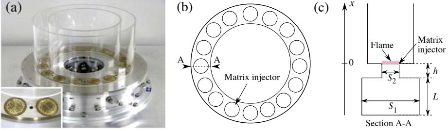
FIGURE 24. (a) MICCA annular combustor equipped with matrix laminar injectors. (b) Top view of showing the 16 matrix injectors. (c) Cut A-A view with the main dimensions. Adapted from Bourgooin et al. (2015).
