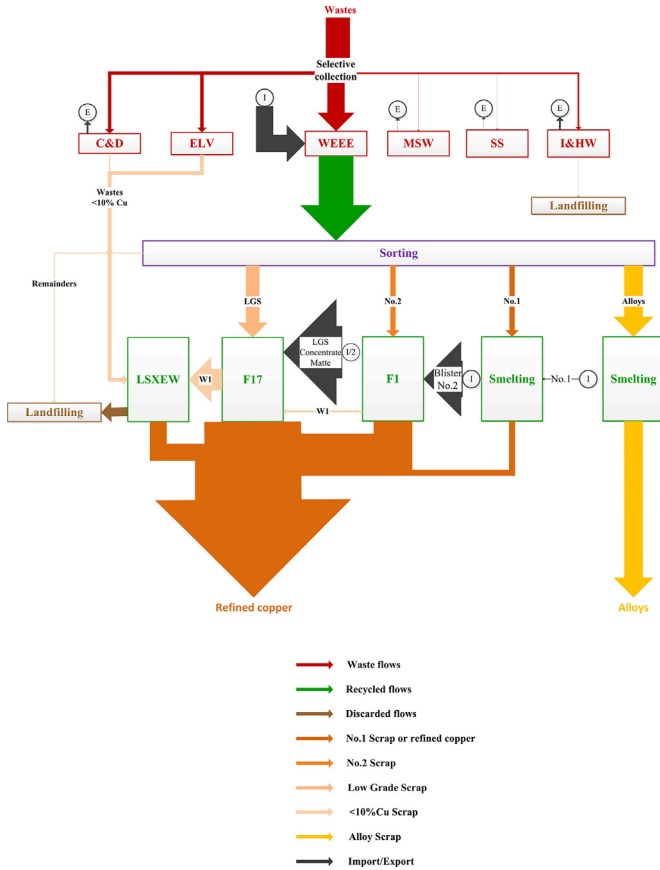
Fig. 13. Representation of flows for the compromise solution obtained with biobjective optimization.
