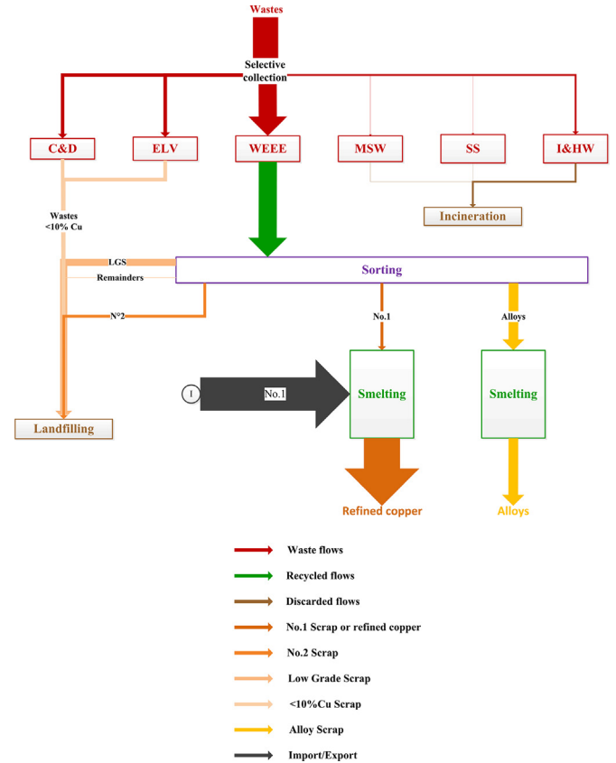
Fig. 7. Representation of flows during minimization of the energy consumption.
