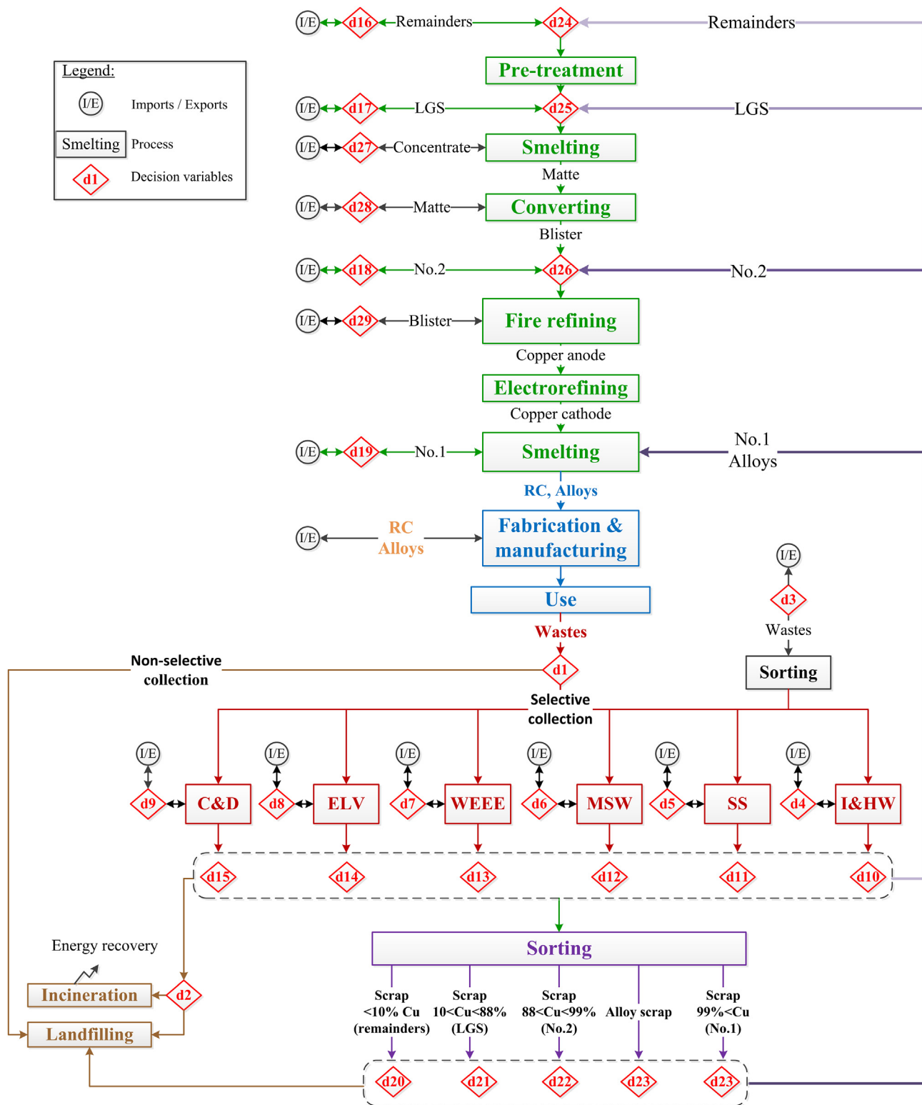
Fig. 1. Superstructure of copper processing pathways.
