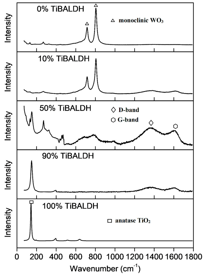
Figure 8. Raman spectra of the fibers after annealing.
