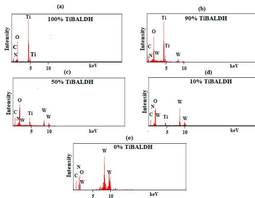
Figure 5. Energy-dispersive X-ray (EDX) spectra of the annealed fibers: (a) 100% TiBALDH, (b) 90% TiBALDH, (c) 50% TiBALDH, (d) 10% TiBALDH, and (e) 0% TiBALDH.
