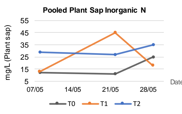
Figure 2 Plant Sap Inorganic Nitrogen Concentration, in the oldest and less defected leaves of Pak choi plants sampled from each treatment. Each data point shows the concentration of total N from a pool of approx. 100 leaves.
