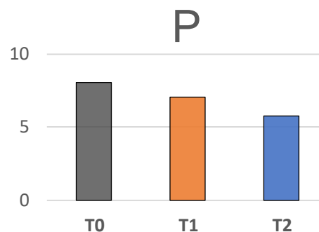
Figure 8 Ratio of averaged plant sap phosphorus to postharvest soil remaining phosphorus , computed by taking the mean concentration of plant sap phosphorus from plants grown in each treatment and divide those means with the postharvest soil remaining P concentration of each treatment. The highest difference of this sap-to-soil ratio was shown for T0 (plants grown in control soil without added fertilisers). This shows that T0 plants grown in the lowest relative soil concentration of P were able to accumulate the highest relative sap concentration of P (see Discussion).
