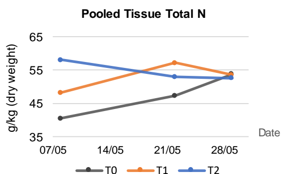
Figure 1 Leaf Tissue Total Nitrogen Concentration, in the youngest fully developed leaves of Pak choi plants sampled from each treatment on three occasions. Each data point shows the concentration of total N from a pool of approx. 100 leaves.
