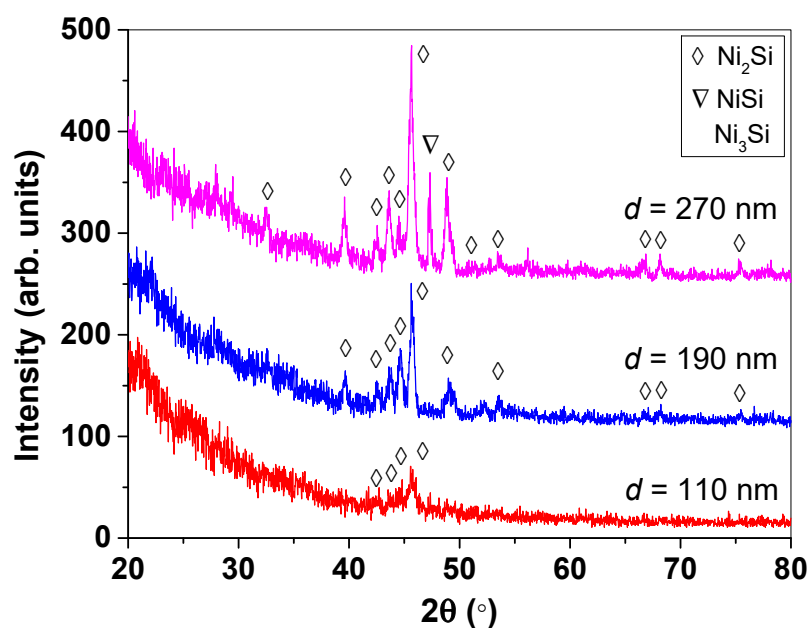
Figure 4. XRD patterns of the NiSi/SiC core-shell nanowires grown by HWCVD at different Ni thicknesses of 110, 190, and 270 nm. The legend indicates the phases of the NiSi chemical formula.
