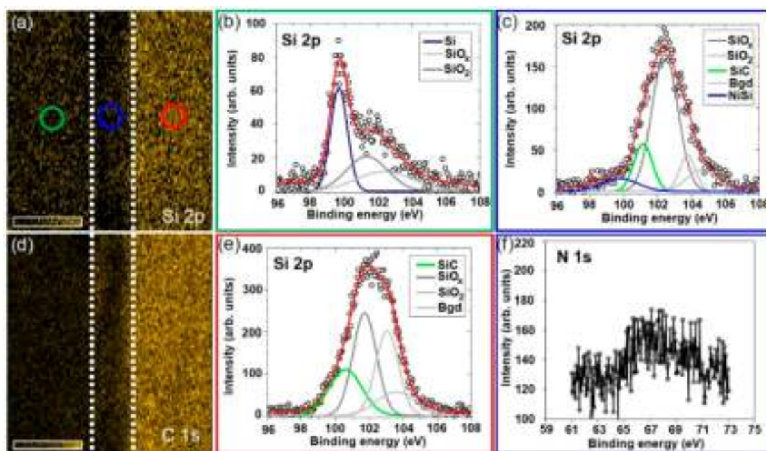
Figure 6. (a,d) XPS map images of Si 2p and C 1s of NiSi/SiC core-shell nanowires grown by HWCVD, respectively. The Si 2p signal was collected by a higher binding energy detector. The brightness of the map images is relatively corresponding to the intensity of the XPS signals (Si 2p and C 1s). The pixel size is approximately 2 \times 2 \mu\text{m}^2 . (b,c,e) The respective XPS narrow-scans of Si 2p at the position in (a) indicated by the empty circle with different colors. (f) The respective XPS narrow-scan of Ni 3p at the position in (a) as indicated by the blue color of the empty circle.
