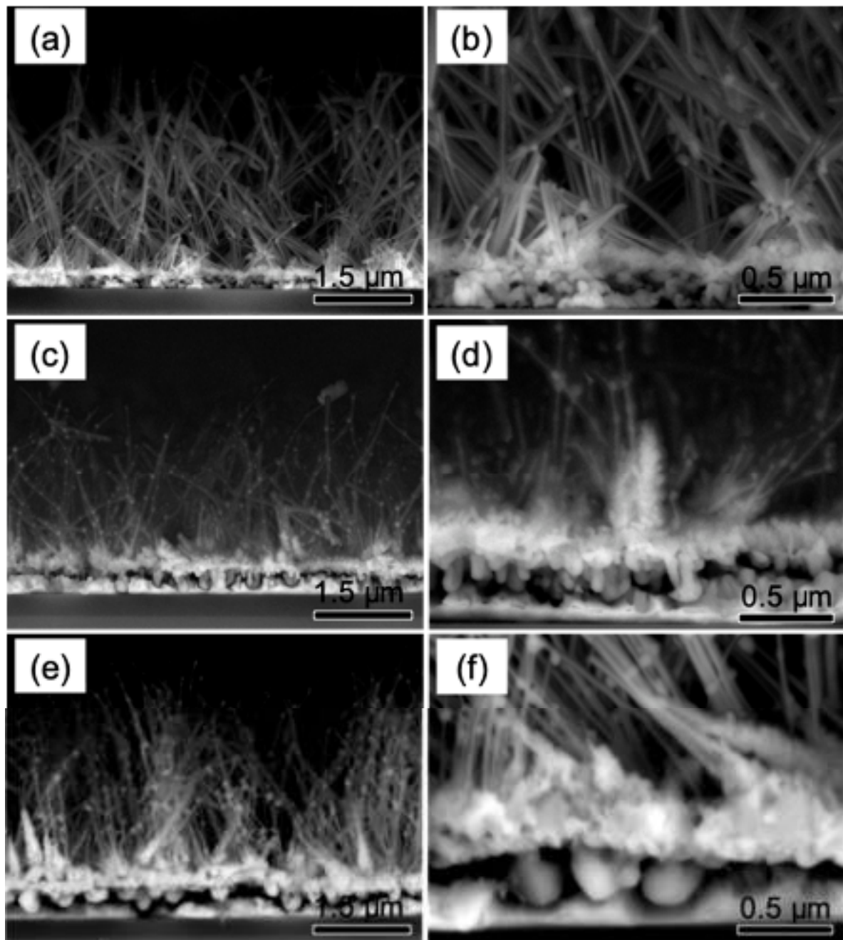
Figure 2. FESEM cross-section images of NiSi/SiC core-shell nanowires grown by HWCVD on c-Si substrate at different Ni thicknesses of 110, 190, and 270 nm. The FESEM images scanned at low magnification (a,c,e) and the respective images scanned at high-magnification (b,d,f) by using photodiode-backscattered electron (PDBSE) detector.
