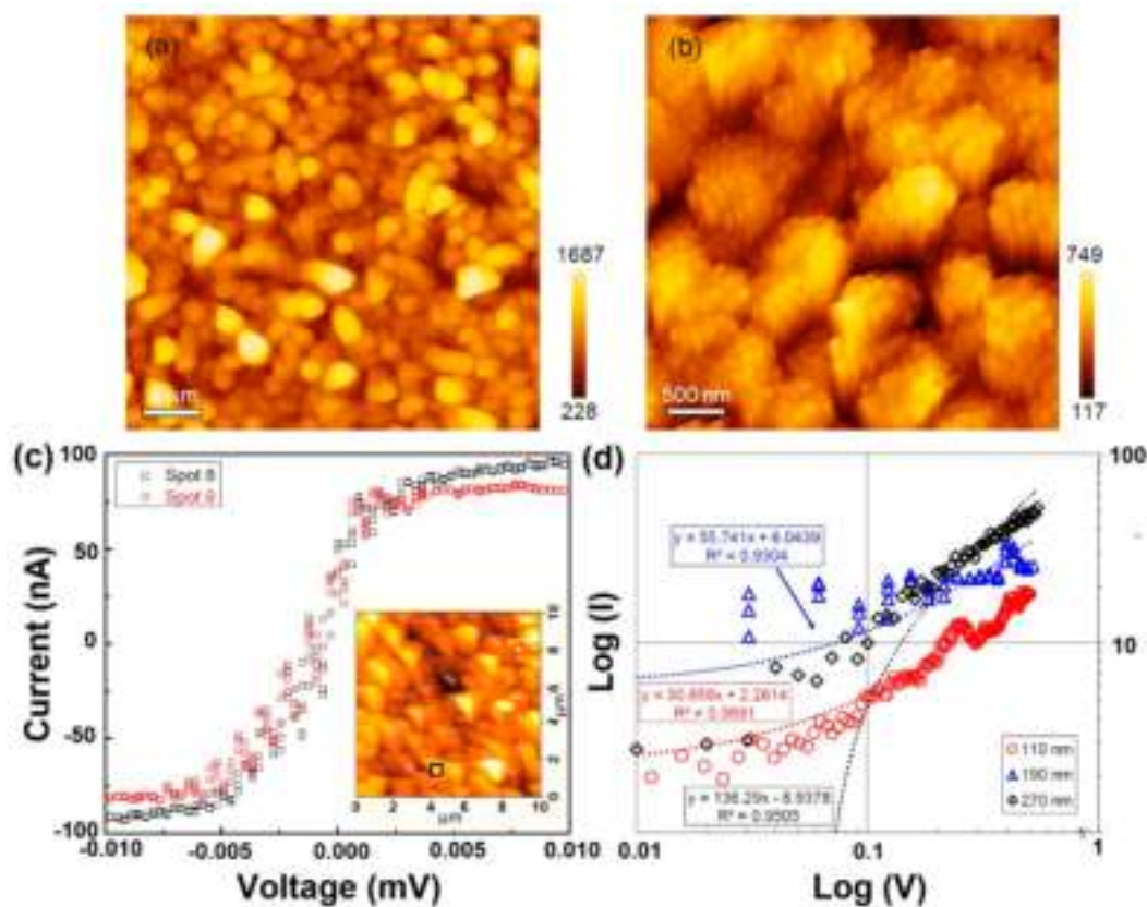
Figure 9. (a,b) Atomic Force Microscopy (AFM) images of the NiSi/SiC core-shell nanowires grown by HWCVD. (c) Current–voltage curves of the nanowires obtained at different spots with the positions as shown in inset of the conducting AFM image. (d) Current–voltage curves of the nanowires at different spots in the Ohmic regions.
