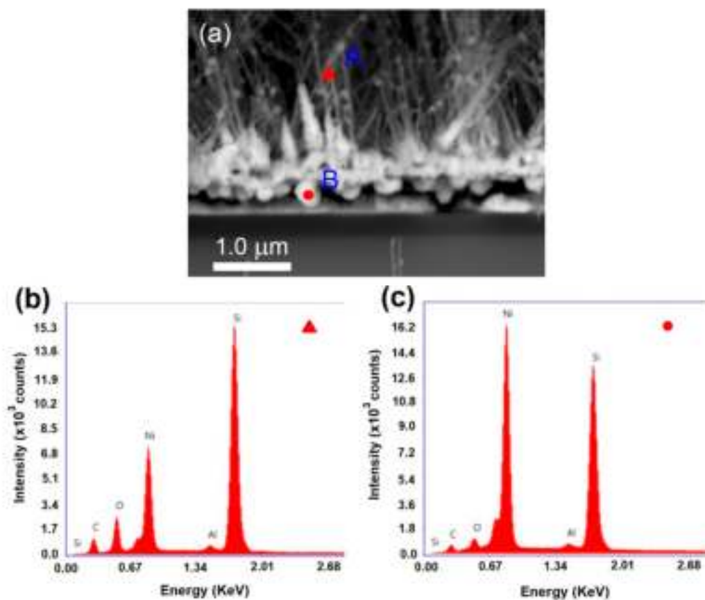
Figure 3. (a) The FESEM cross-section image of the nanowires scanned by PDBSE detector. (b,c) energy-dispersive X-ray (EDX) spectra obtained at the stem of nanowires (marked as A) and at the solid particle between the deposition layer and c-Si substrate (marked as B) respectively as labelled in (a).
