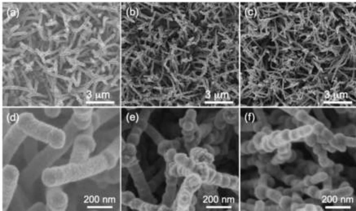
Figure 1. Field emission scanning electron microscopy (FESEM) images of the NiSi/SiC core-shell nanowires grown by hot-wire chemical vapor deposition (HWCVD) at different Ni thicknesses of (a,d) 110, (b,e) 190, and (c,f) 270 nm. The top and bottom images represent low and high magnifications of the micrograph images, respectively.
