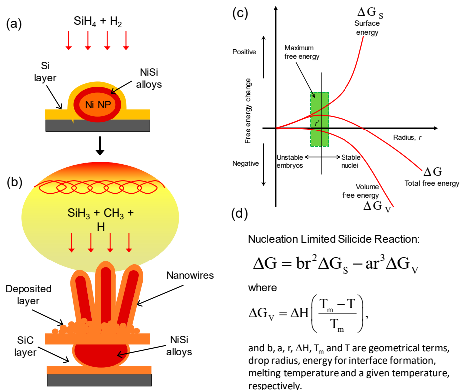
Figure 8. (a,b) Growth mechanisms of the NiSi nanoparticle and NiSi/SiC core-shell nanowires grown by HWCVD, respectively. (c) Free energy changes as function of drop radius for NiSi reactions. The shadowed region is proposed as a region for the growth of NiSi core nanowires. (d) The nucleation limited silicide reaction relation for the growth of the core nanowires.
