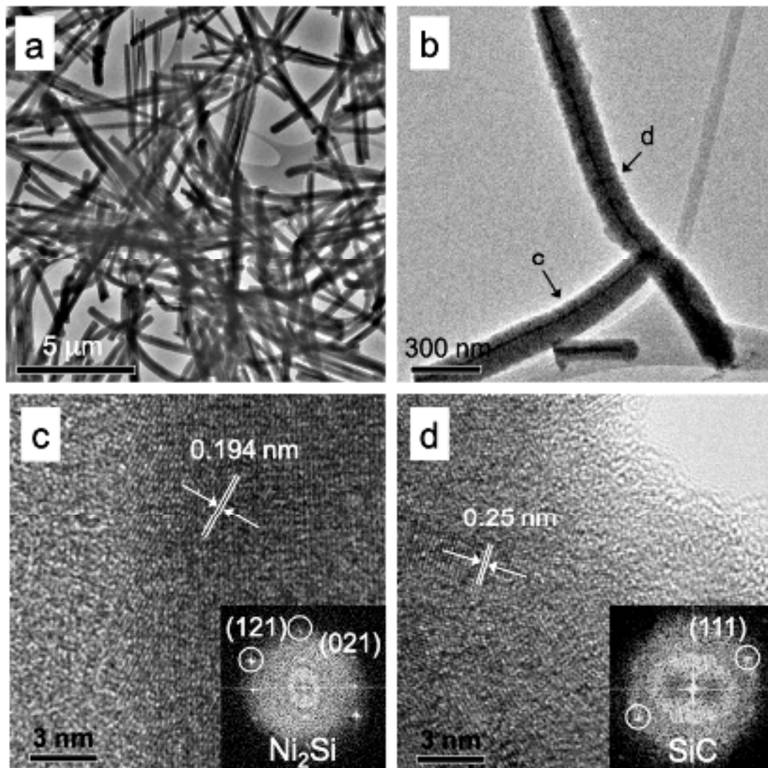
Figure 7. (a) Typical TEM image of nanowires grown by HWCVD. (b) TEM image of a branched nanowire grown by HWCVD. (c,d) High-resolution TEM images taken on the nanowire where the positions are indicated by the arrows as shown in (b). Insets (c,d) represent the FFT images of the core and shell of the nanowire respectively.
