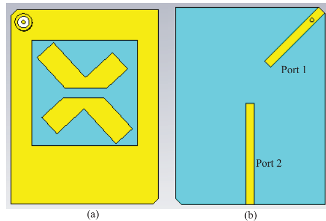
Figure 2: Dual circular-polarized slot antenna, Design 2-A (a) Forward-facing view (b) Opposite view
