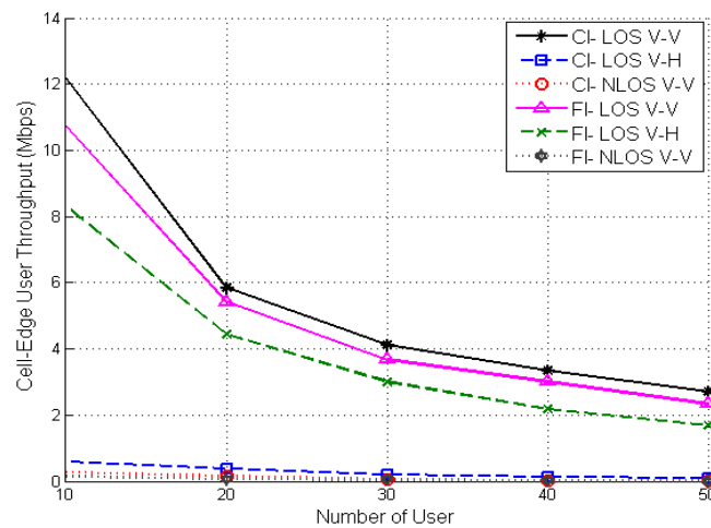
Figure 8. Cell-edge user throughput vs number of users.
