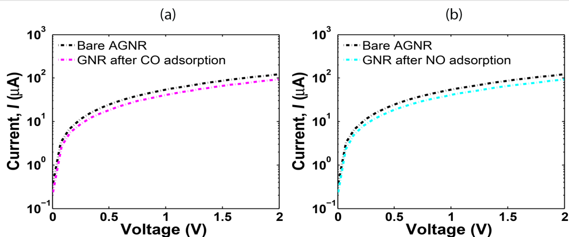
Figure 6: Armchair graphene nanoribbon (AGNR) sensor I - V characteristics obtained using the Atomistix Toolkit (ATK): (a) after CO and (b) after NO.
